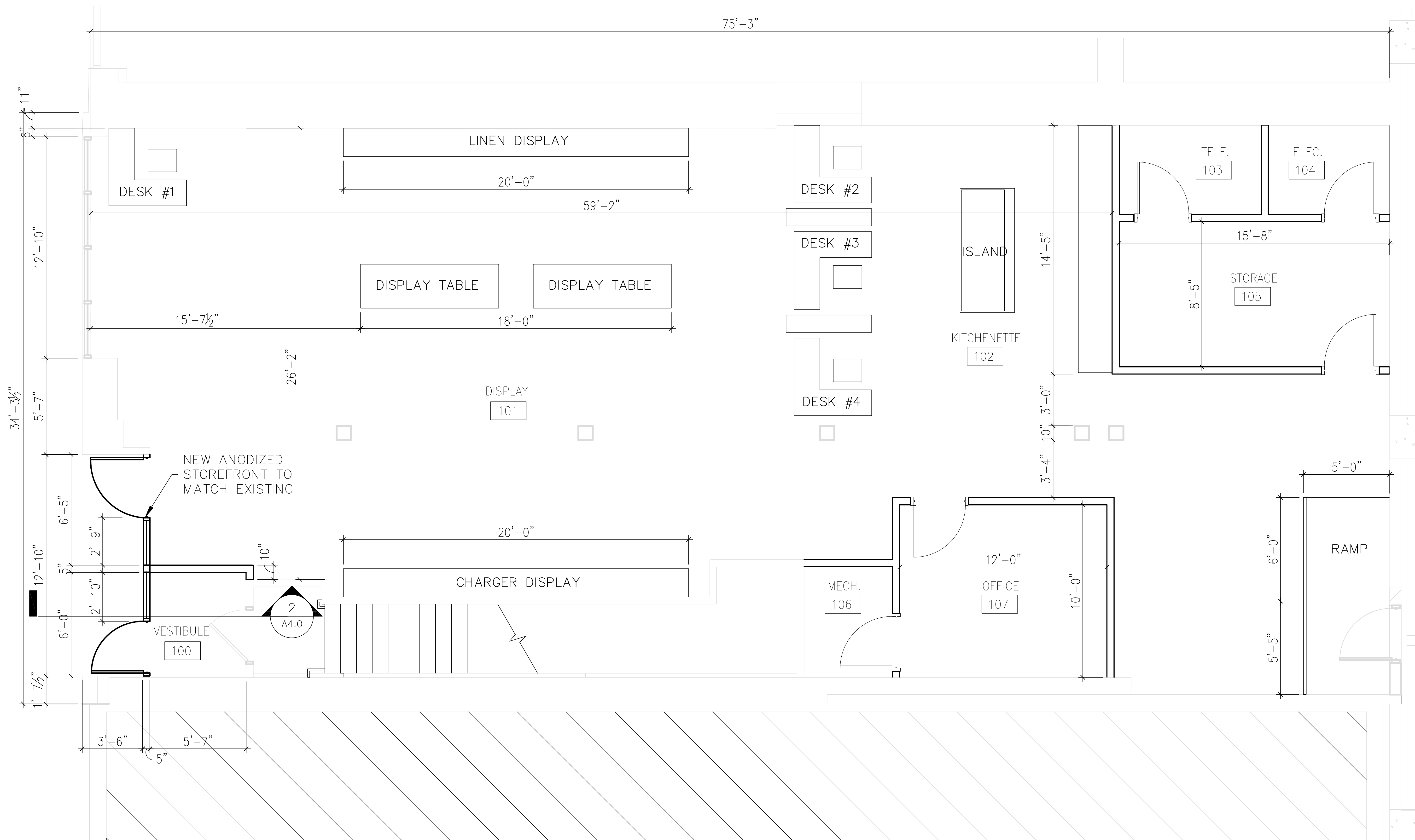
1 FIRST FLOOR PLAN 3/8" = 1'-0"
