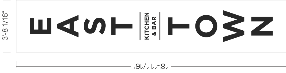
GRAPHIC DETAIL SCALE: 1/4" = 1'-0"
