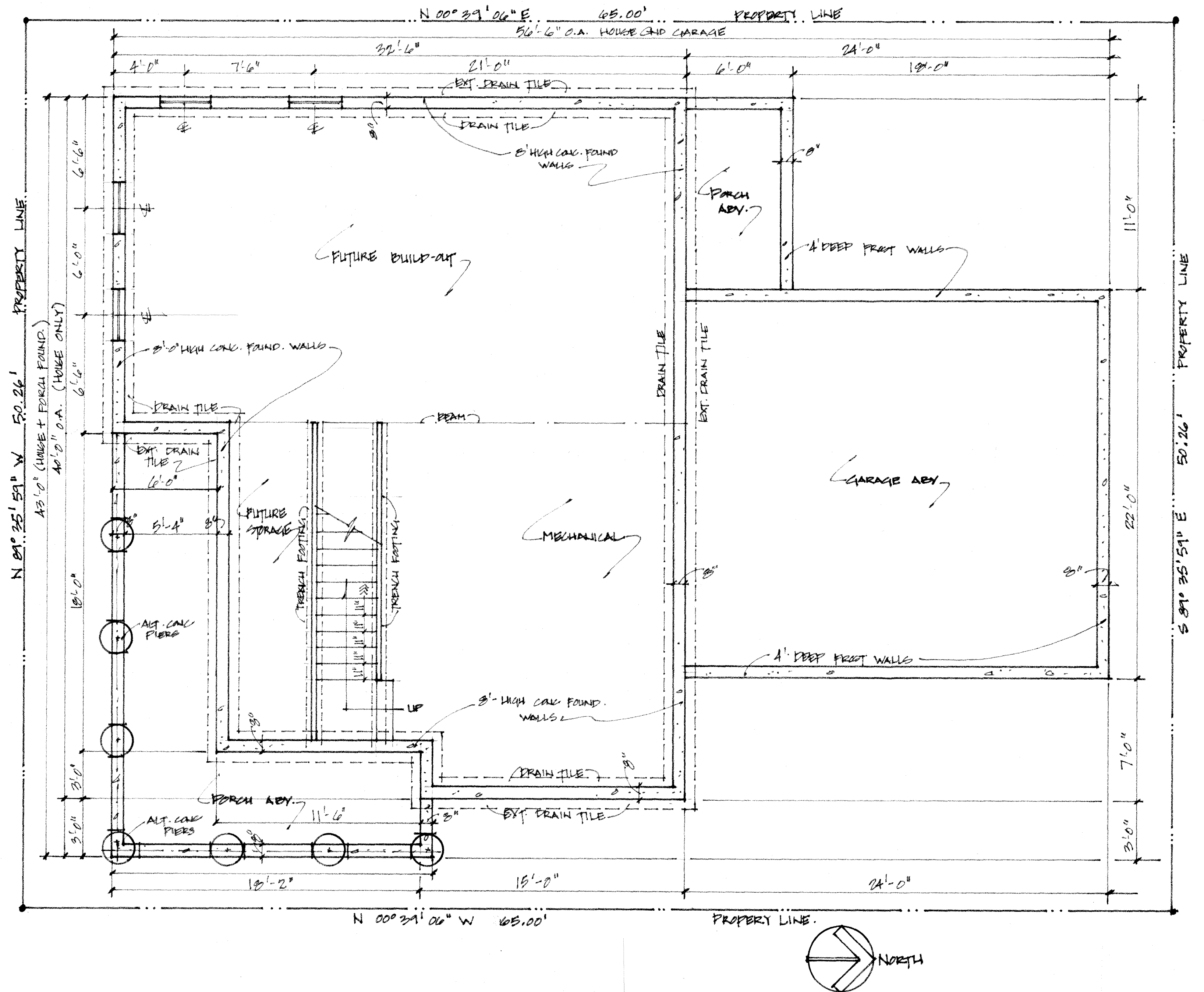
LOWER LEVEL / FOOTINGS & FOUNDATION PLAN 1/4" = 1'-0"
