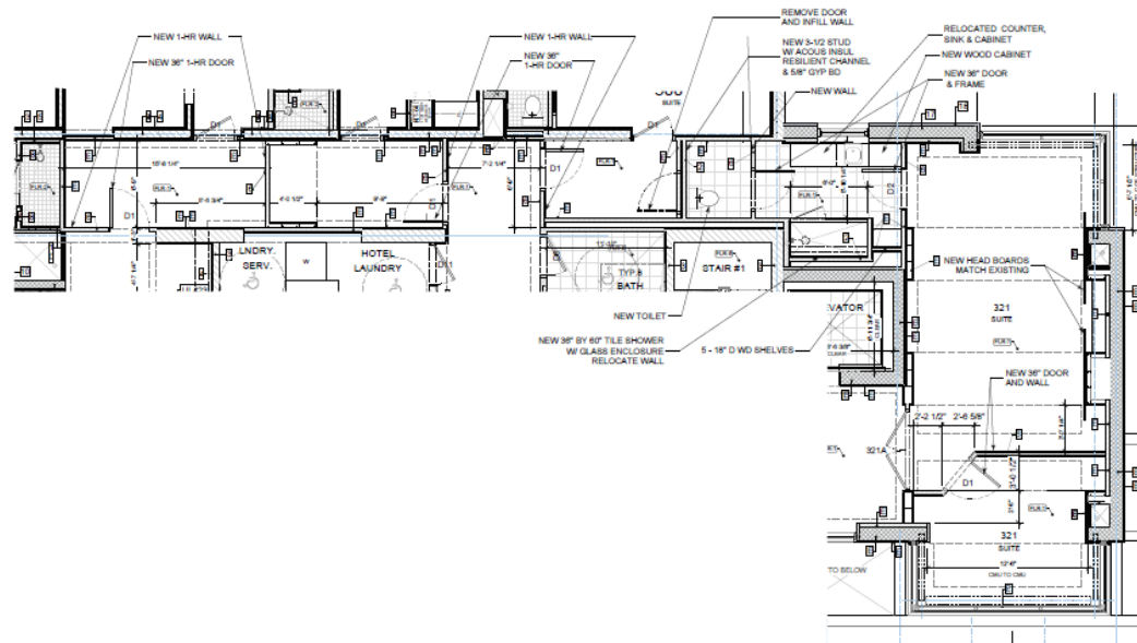
1 Partial Third Floor Plan 1/4" = 1'-0"
