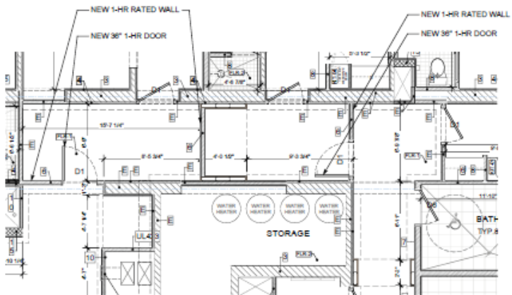
3 Partial Second Floor Plan 1/4" = 1'-0"
