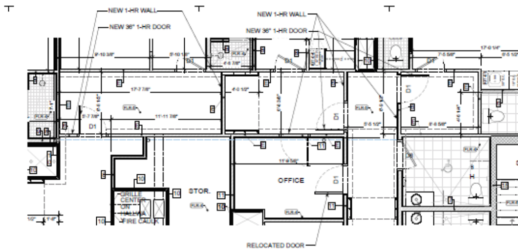
2 Partial Fourth Floor Plan 1/4" = 1'-0"
