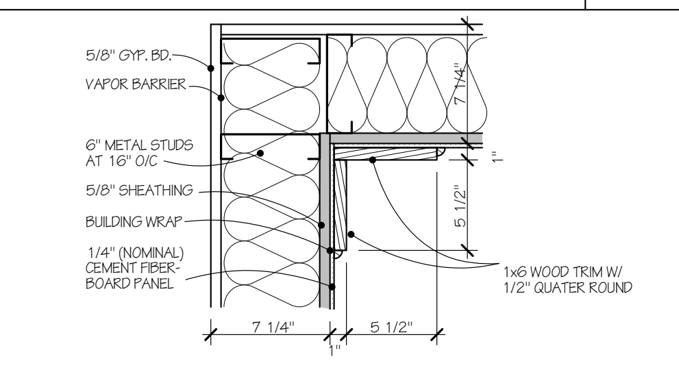
WALL DETAIL 1 1/2" = 1'-0" 1 0
