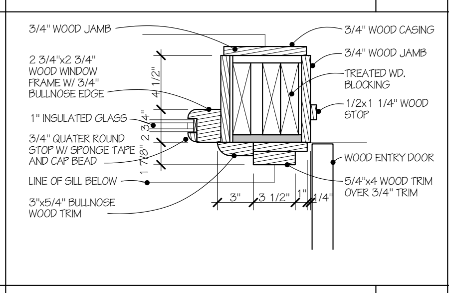
WINDOW JAMB DETAIL 1 1/2" = 1'-0" 1 3
