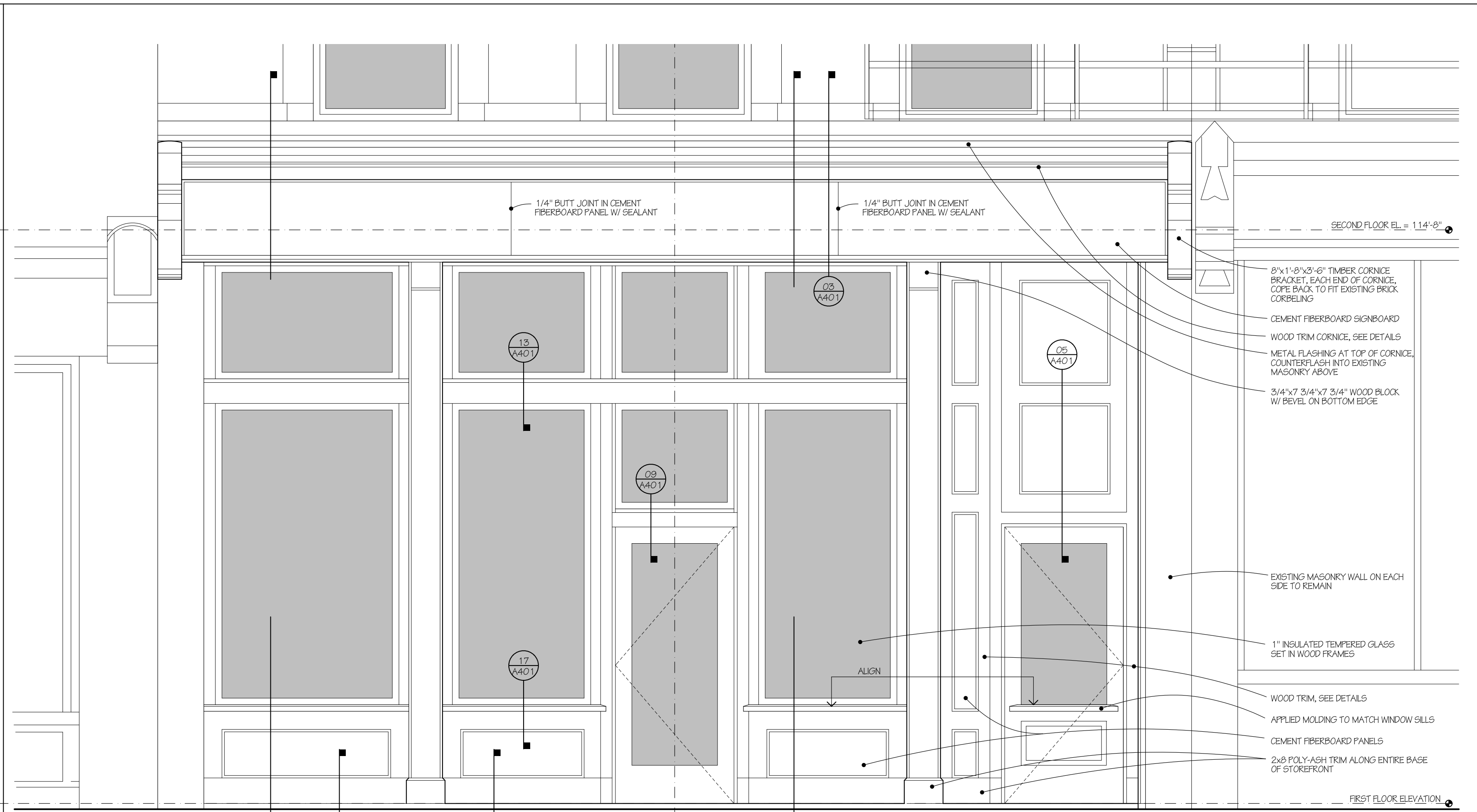
PARTIAL EAST ELEVATION 1/2" = 1'-0" 0 3
