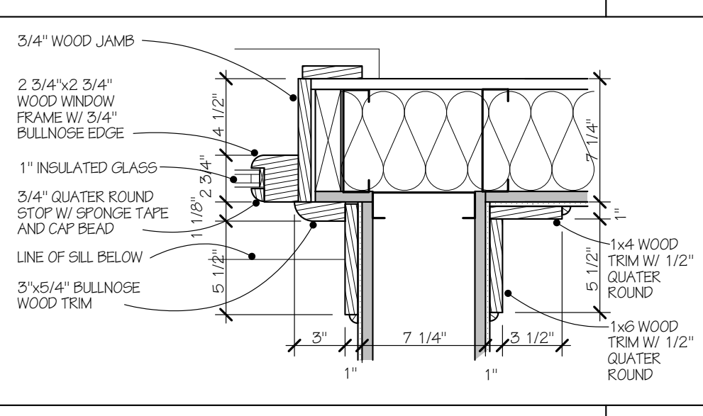
WINDOW JAMB DETAIL 1 1/2" = 1'-0" 0 9
