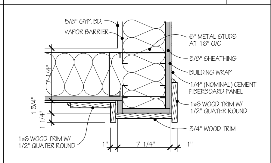
WALL DETAIL 1 1/2" = 1'-0" 1 4
