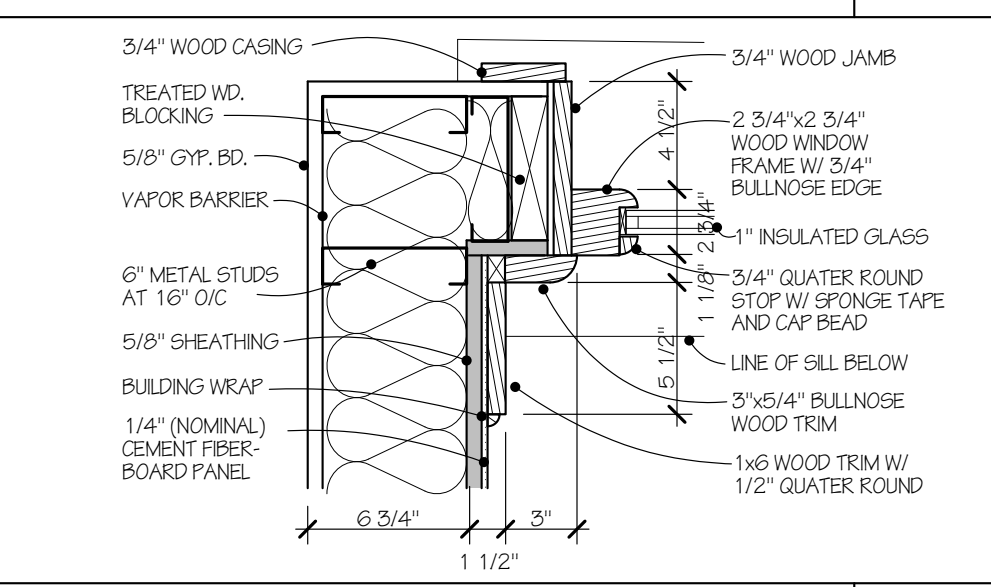
WINDOW JAMB DETAIL 1 1/2" = 1'-0" 1 1
