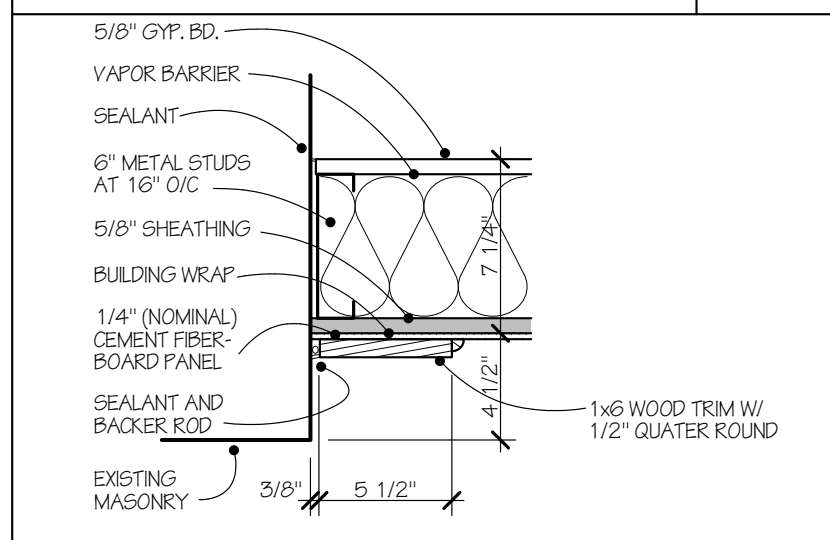
WALL DETAIL 1 1/2" = 1'-0" 1 8
