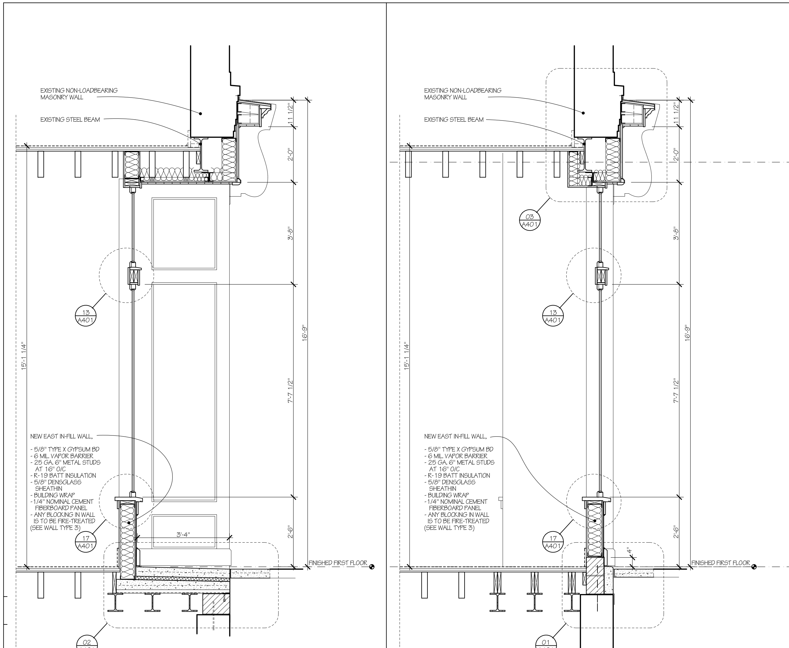
PARTIAL EAST ELEVATION 1/2" = 1'-0" 0 3
