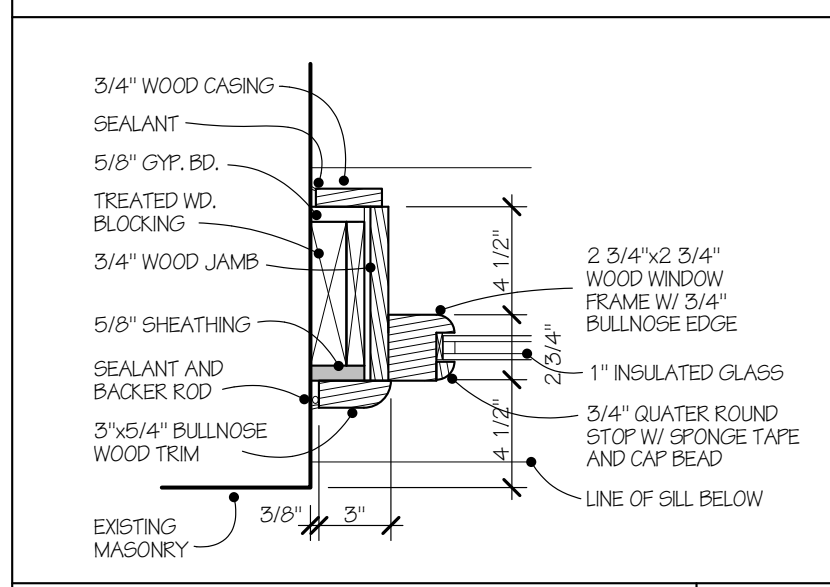
WINDOW JAMB DETAIL 1 1/2" = 1'-0" 1 9
