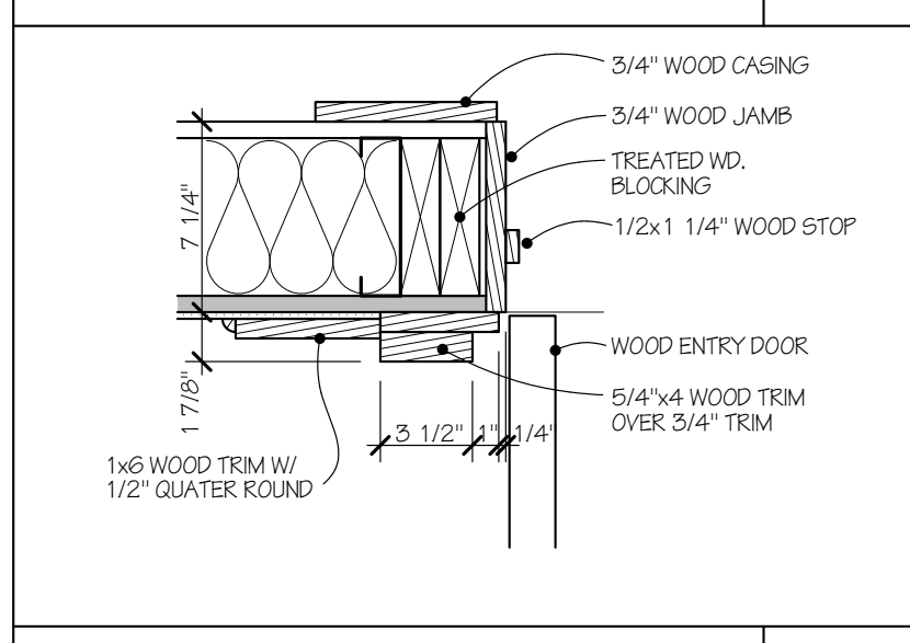
DOOR JAMB DETAIL 1 1/2" = 1'-0" 1 7
