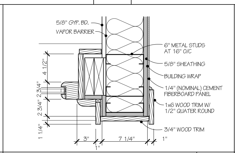
WINDOW JAMB DETAIL 1 1/2" = 1'-0" 1 5
