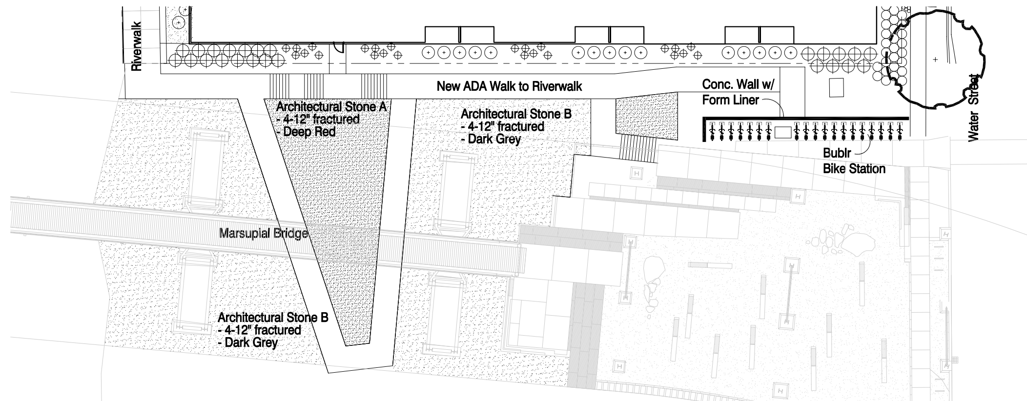
Marsupial Bridge Connection to Riverwalk
