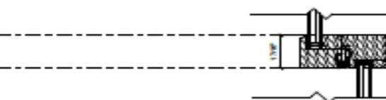
② NEW WOOD WINDOW - MEETING RAIL DETAIL ②' = 1'-0"
