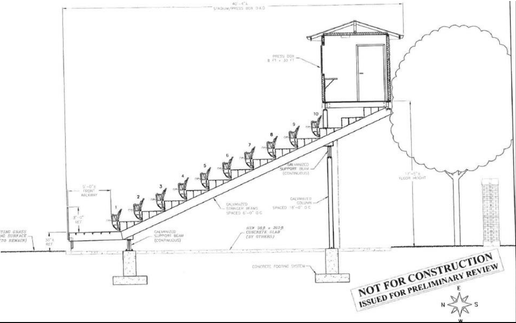
Section through press box
