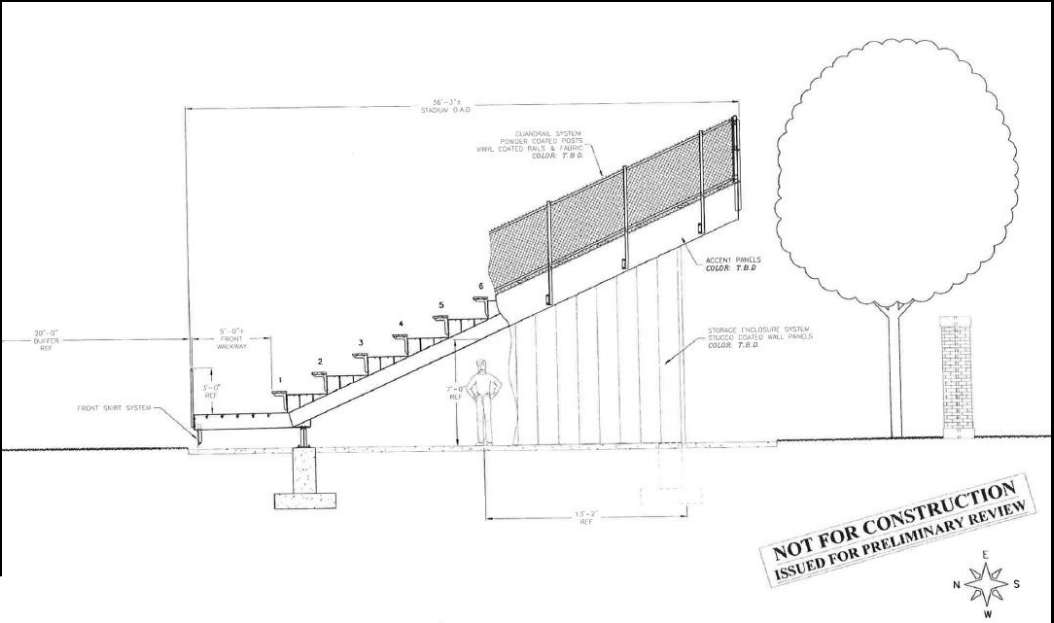
Section through end
