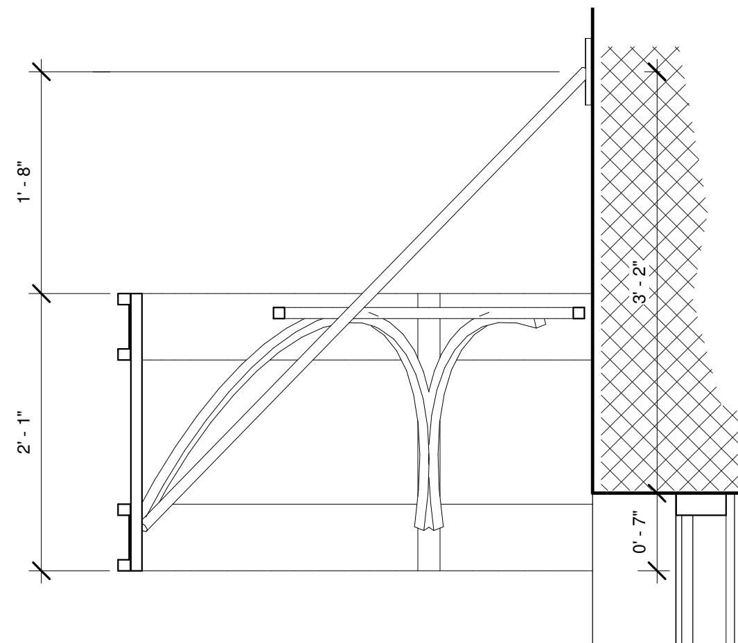
⑤ Section 1 1" = 1'-0"
