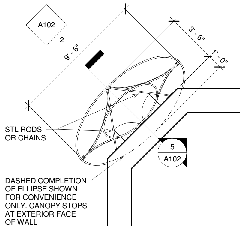
① Canopy Plan 1/4" = 1'-0"
