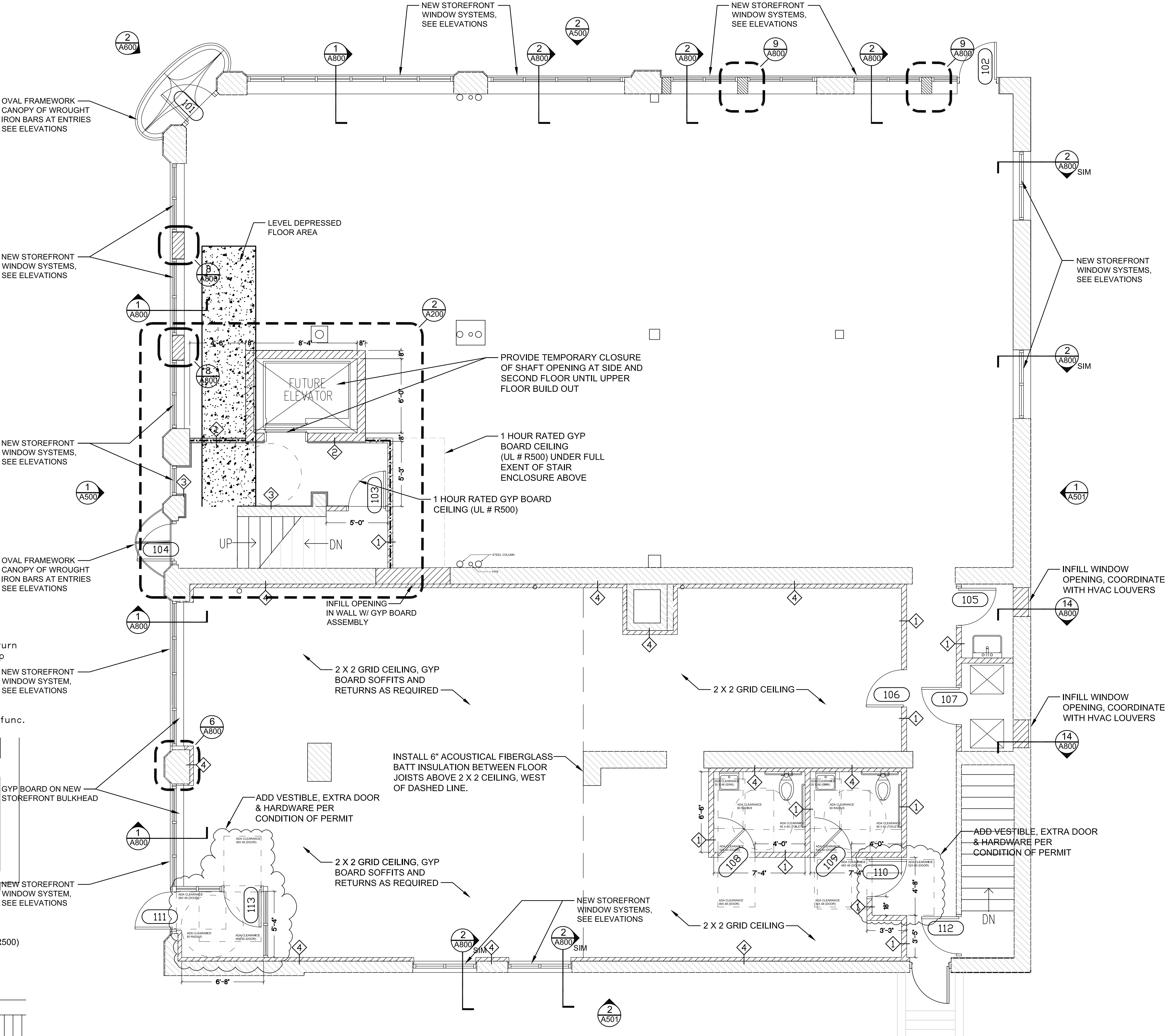
1 FIRST FLOOR NEW PLAN SCALE: 1/4"=1'-0"
