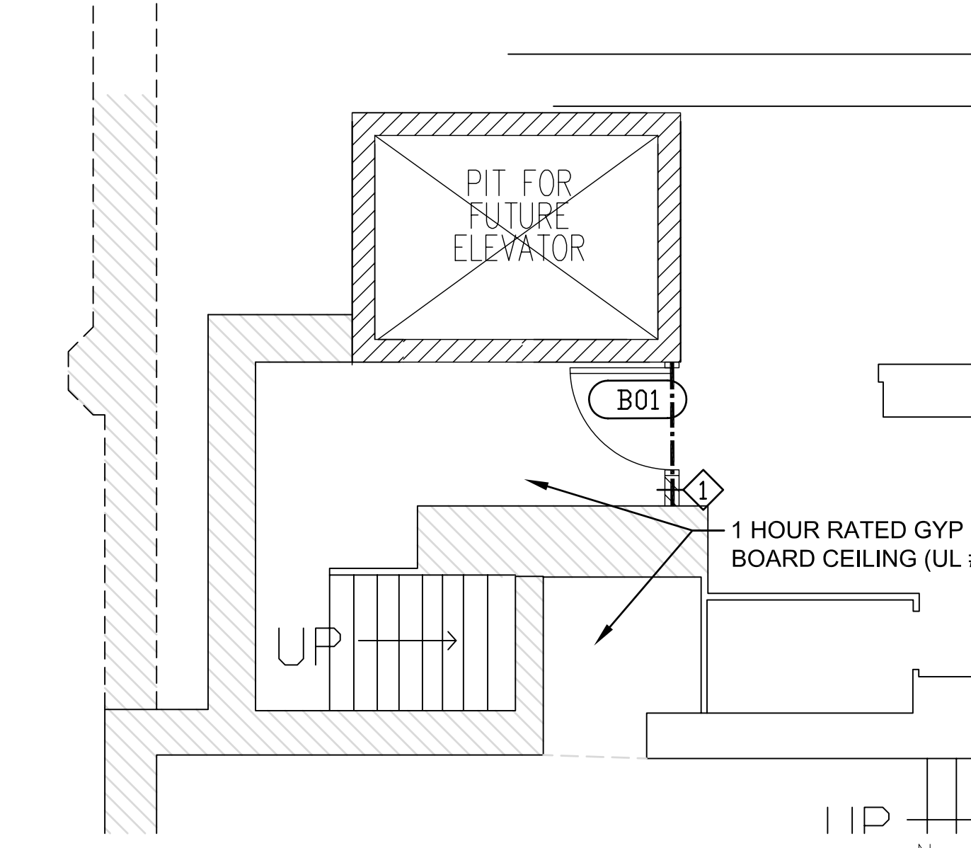
2 ENLARGED PART, BASEMENT PLAN SCALE: 1/4"=1'-0"
