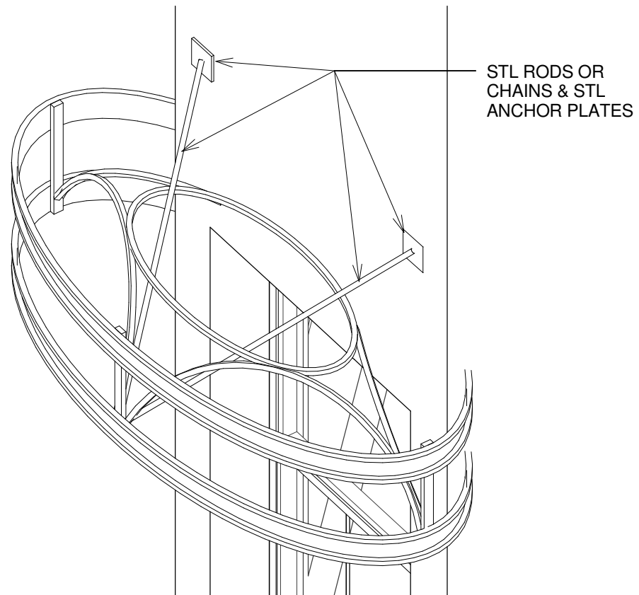
④ Canopy Axon
