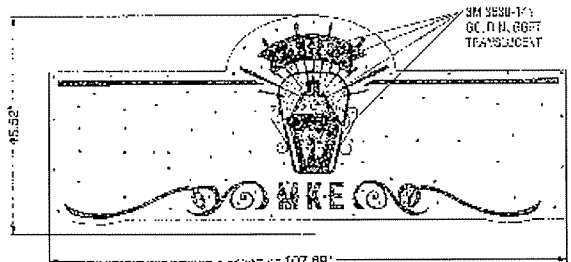
[E] - .125" Thk #7326 Winda Acrylic Backer w/ 1st Surface Applied Vinyl. 3M 3630-141 GOLD NUGGET is translucent. ALL OTHER VINYL IS TO BE OPAQUE.
