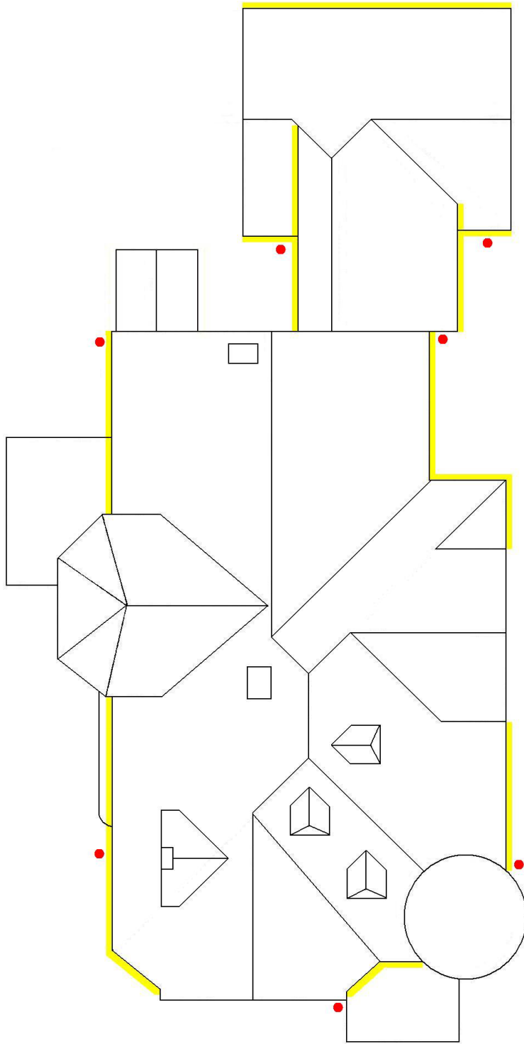
Roof plan with gutters and downspouts. New copper half-round gutters and corrugated copper downspouts will be installed. They will be similar to existing.
