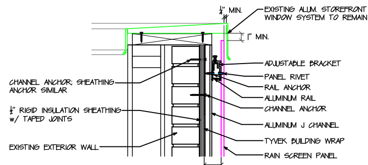
1 PARAPET DETAIL 1/2" = 1'-0"
