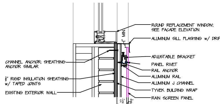
3 WINDOW SILL DETAIL 1/2" = 1'-0"
