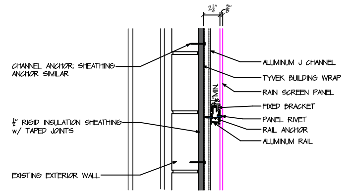
5 HORIZONTAL MID PANEL SUPPORT 1/2" = 1'-0"
