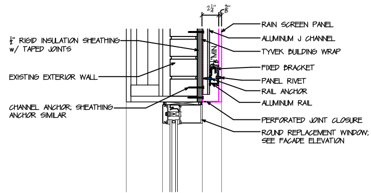
2 WINDOW HEAD DETAIL 1/2" = 1'-0"
