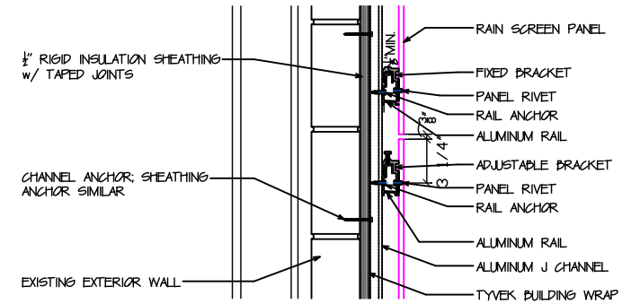
4 HORIZONTAL PANEL JOINT DETAIL 1/2" = 1'-0"
