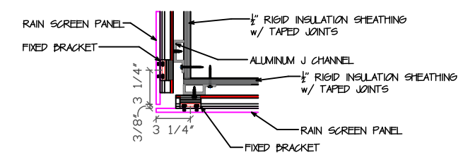
7 OUTSIDE CORNER DETAIL 1/2" = 1'-0"
