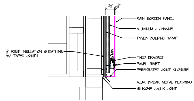
6 BOTTOM TRANSITION CLOSURE 1/2" = 1'-0"
