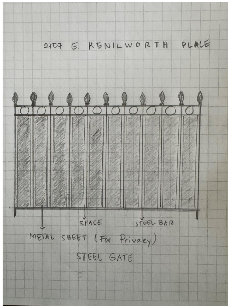
Design of the metal fence/gates
