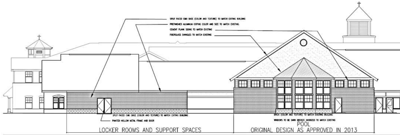
1 NORTH ELEVATION 1/8" = 1'-0"
