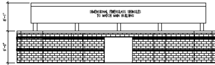
① FRONT OF STAGE ELEVATION 1/4" = 1'-0"
