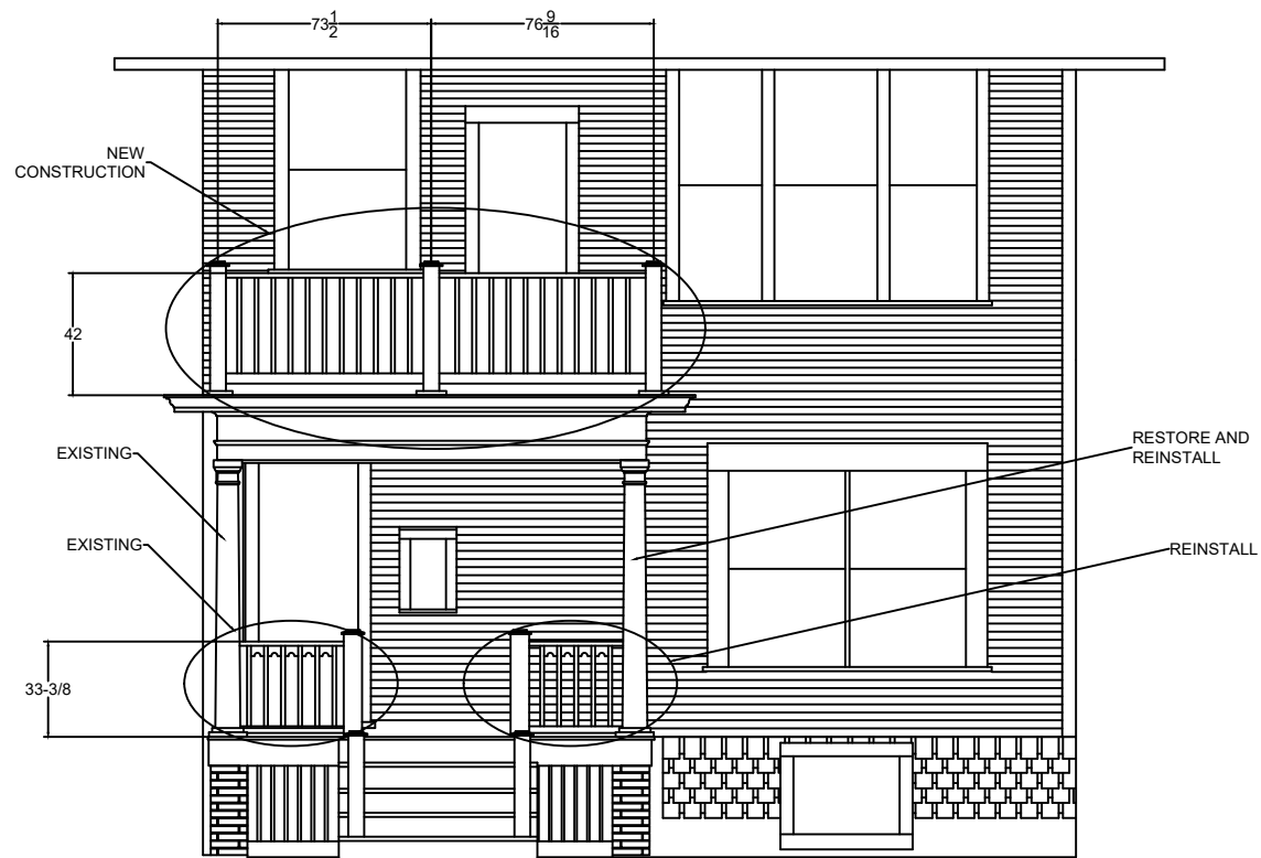
EAST ELEVATION
