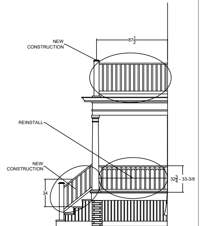
NORTH ELEVATION
