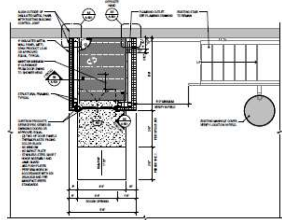
A5 EYE WASH STATION FLOOR PLAN
