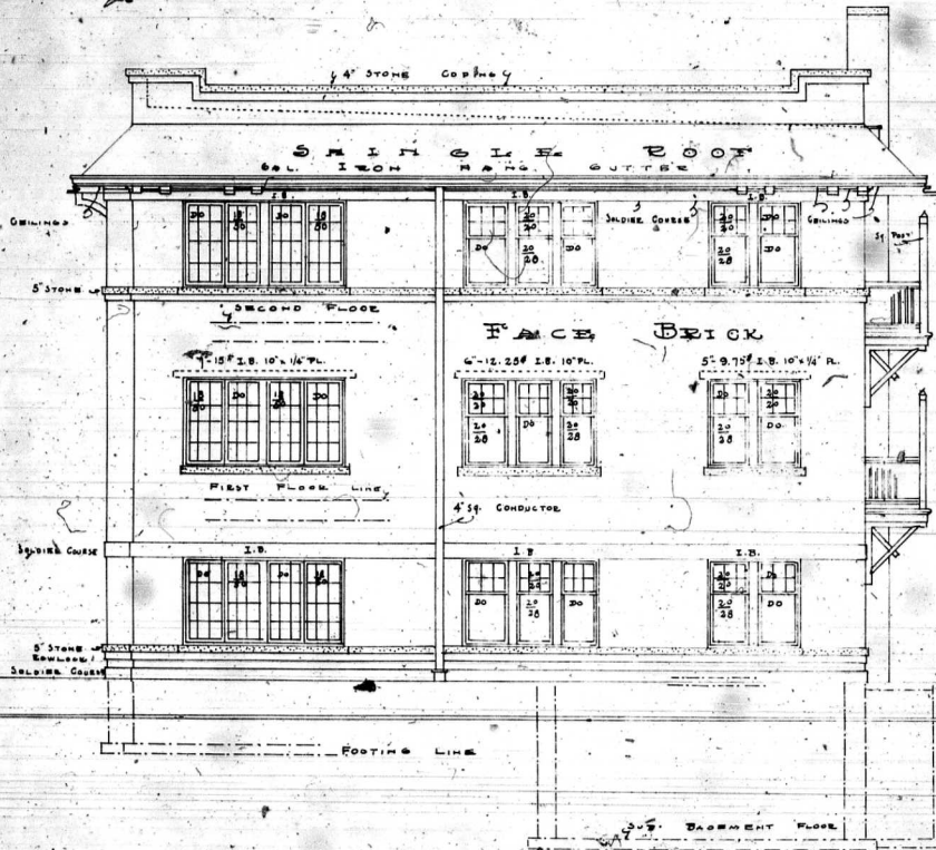
28 TH STR. ELEVATION WM. HOFFMAN
