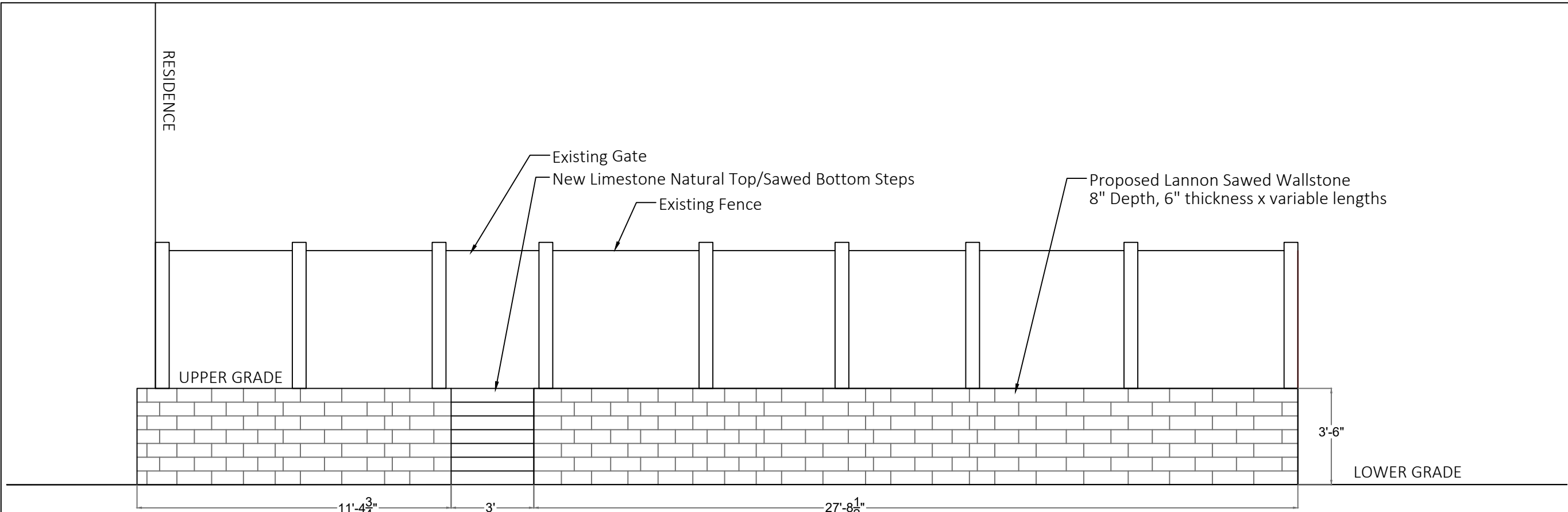
DETAIL - RETAINING WALL
