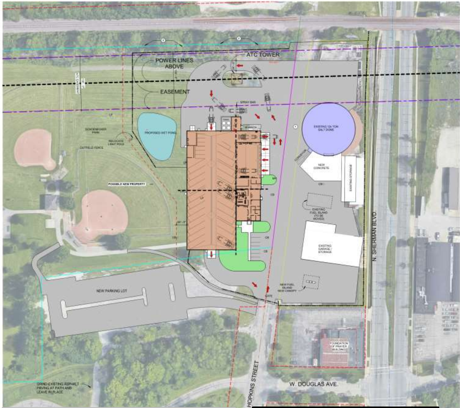
PROPOSED ARCHITECTURAL SITE PLAN
