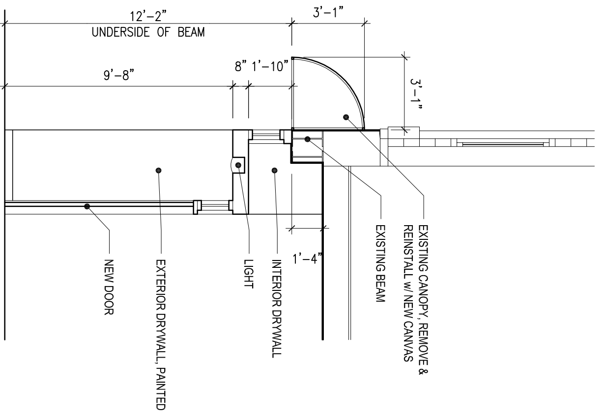
2. SECTION
