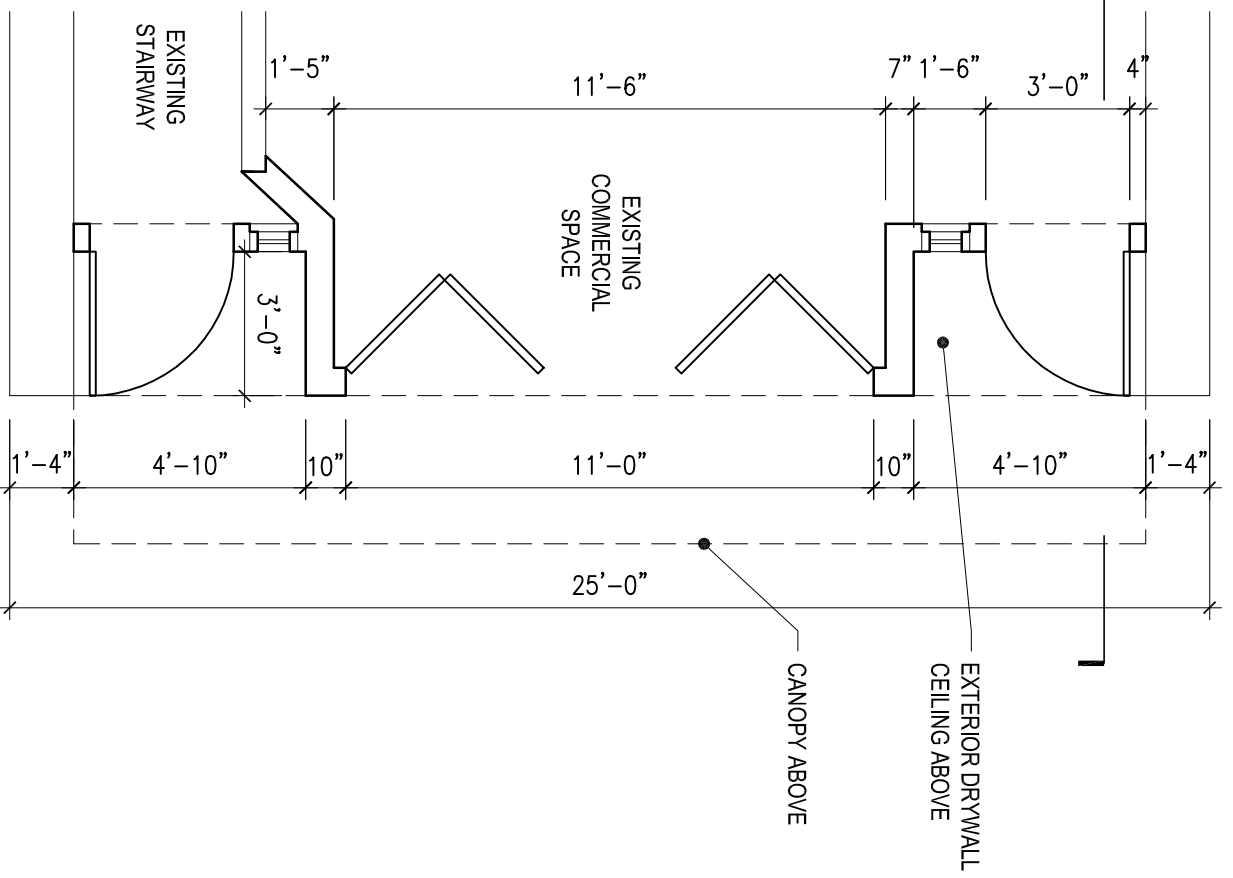
1. PLAN
