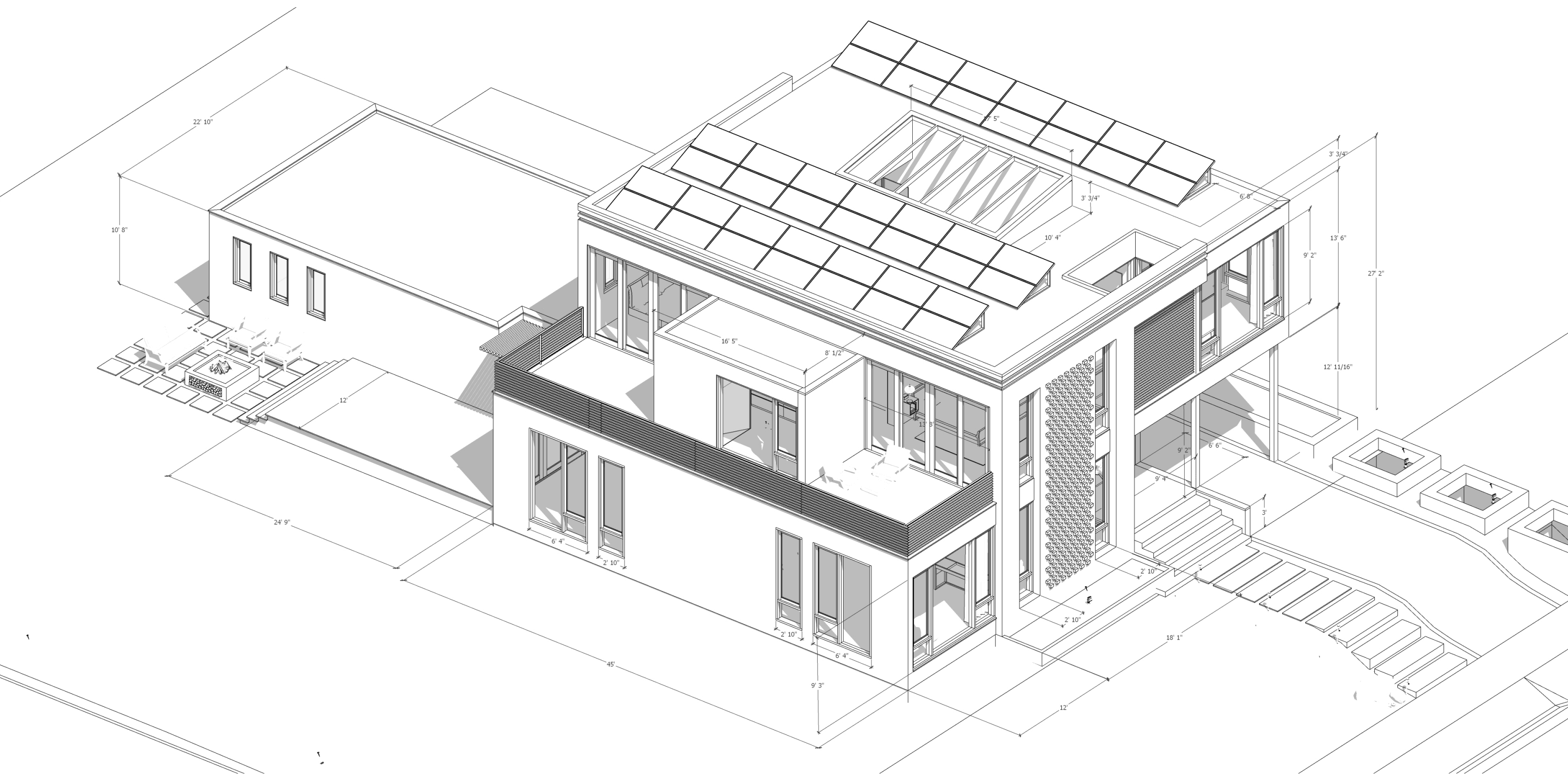
AXONOMETRIC WITH DIMENSIONS
