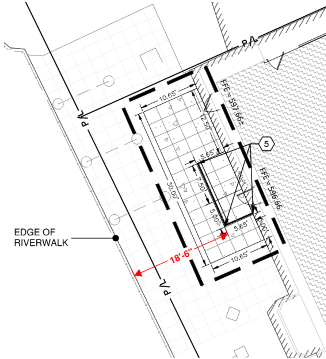
RIVERWALK ACCESS – SITE LAYOUT PLAN
