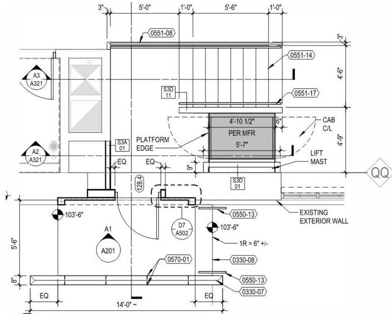
RIVERWALK ACCESS - PLAN
