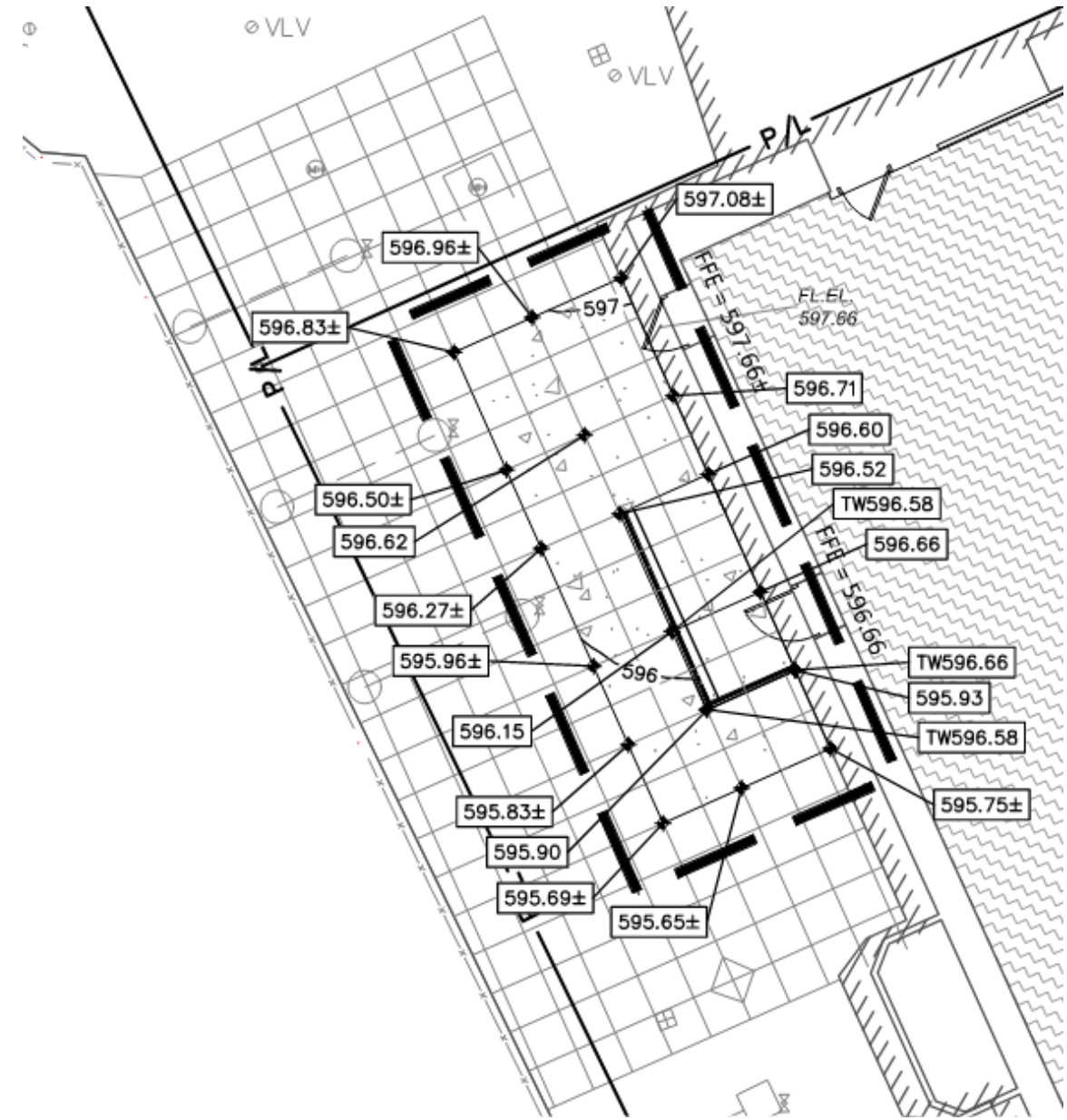
RIVERWALK ACCESS – SITE GRADING PLAN
