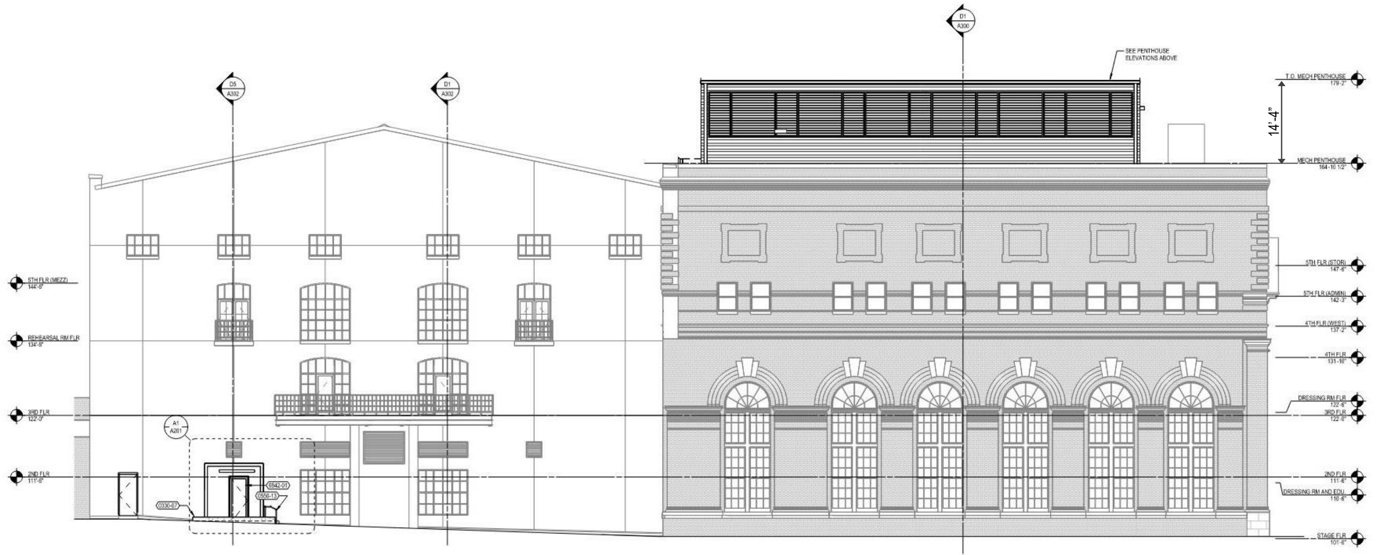
A3 WEST OVERALL ELEVATION 1/8" = 1'-0"
