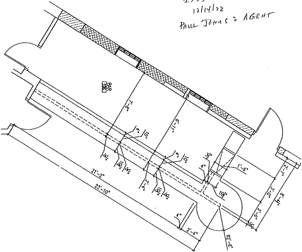
1 A2-00 SCALE - 1/4" = 1'-0" BAR LAYOUT PLAN
