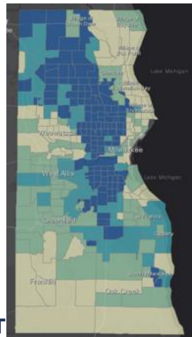
Vulnerability Scores
