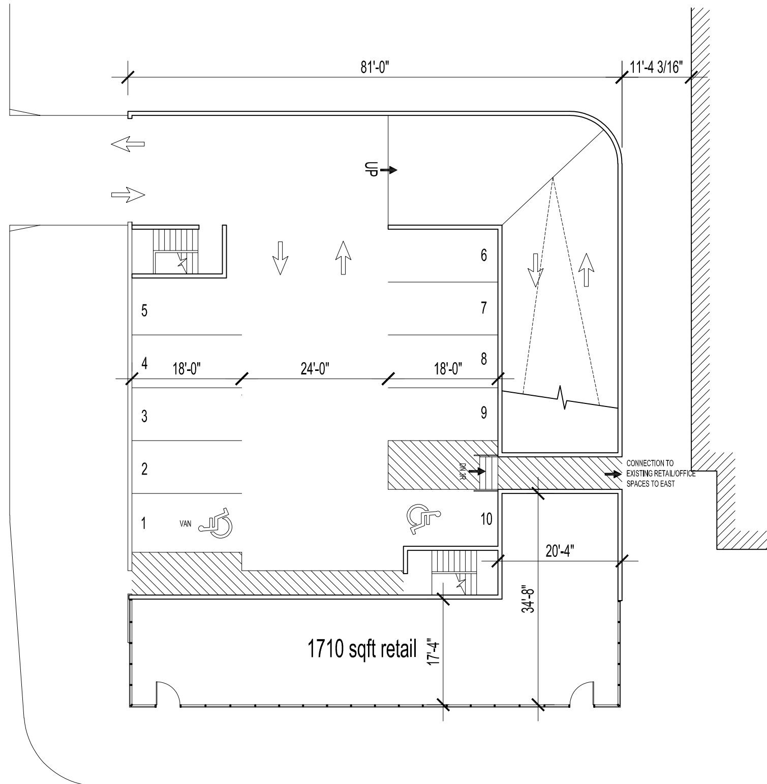
WALNUT STREET LOWER TRAY - 10 STALLS
