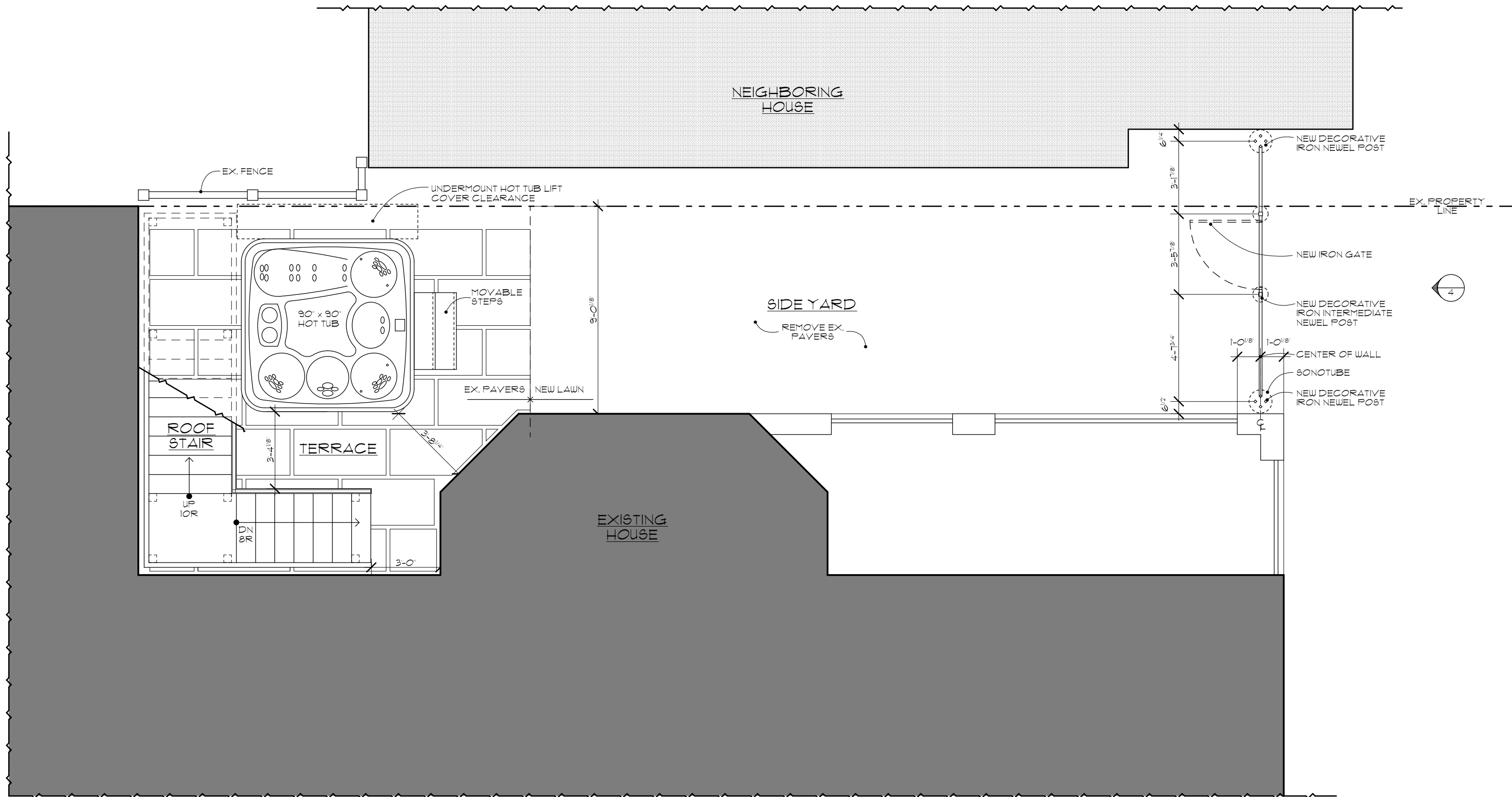
2 HOT TUB AND FENCE PLAN SCALE: 1/4" = 1'-0"
