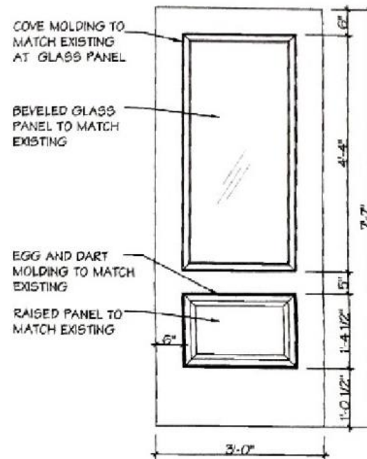
East Door Elevation Scale: 1/2" = 1'-0"
