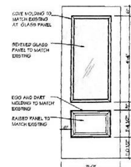
East Door Elevation Scale: 1/2" = 1'-0"
