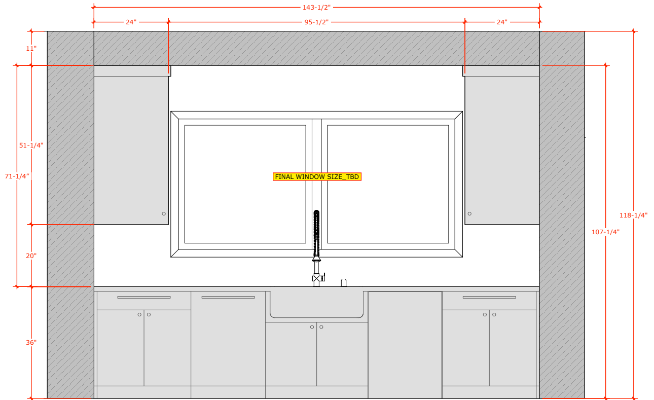
Interior Elevation
