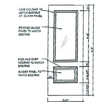
East Door Elevation Scale: 1/2" = 1'-0"
