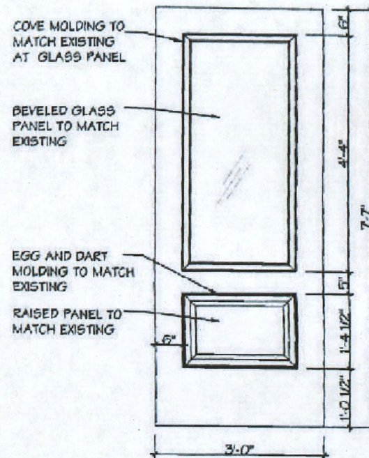
East Door Elevation Scale: 1/2" = 1'-0"
