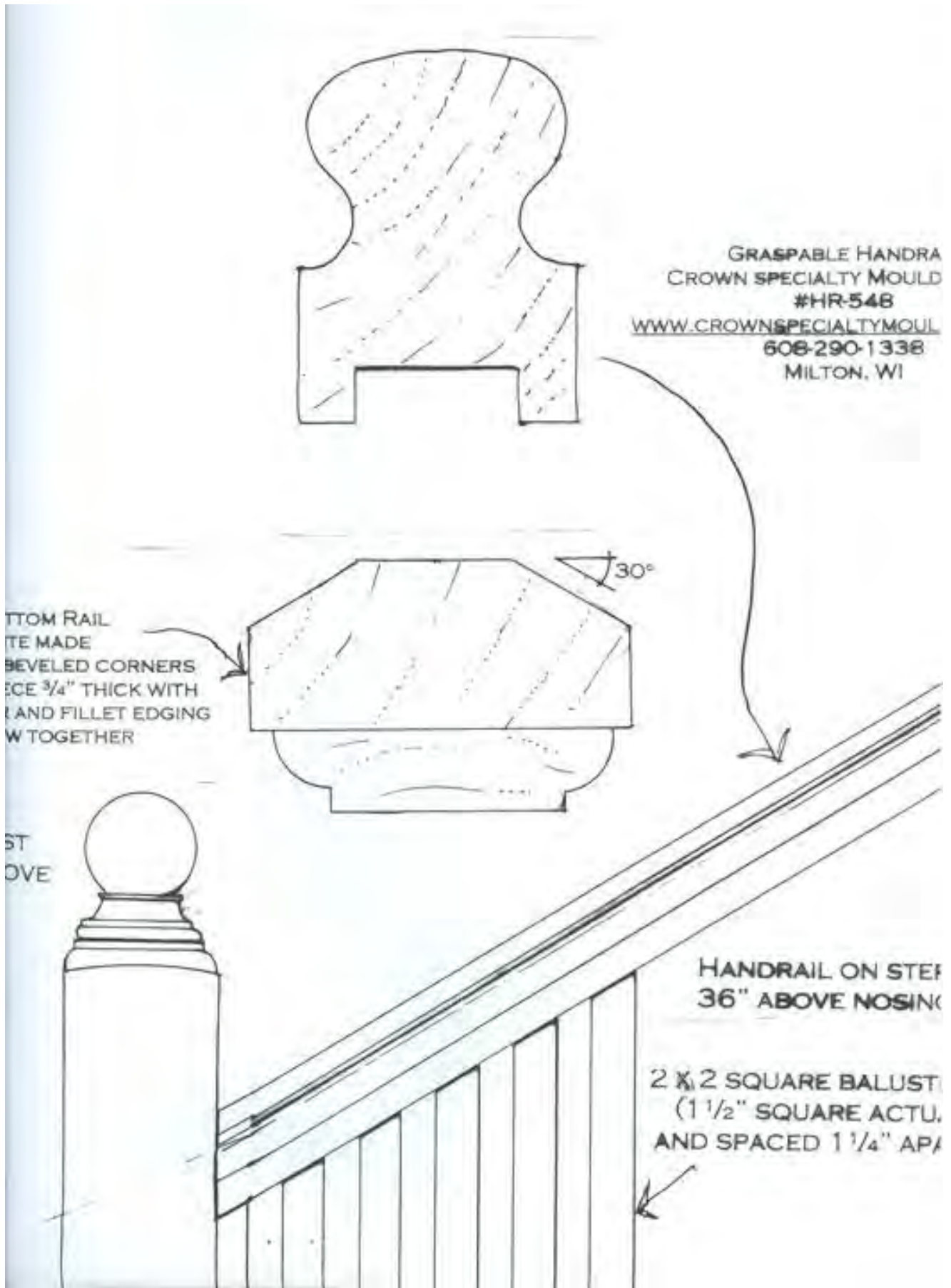
Example of railing elements to be used.
