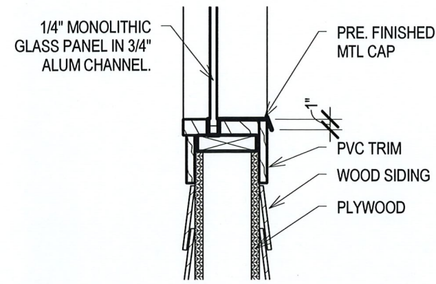
3 DTL AT WNDW SILL Scale: 1" = 1'-0"
