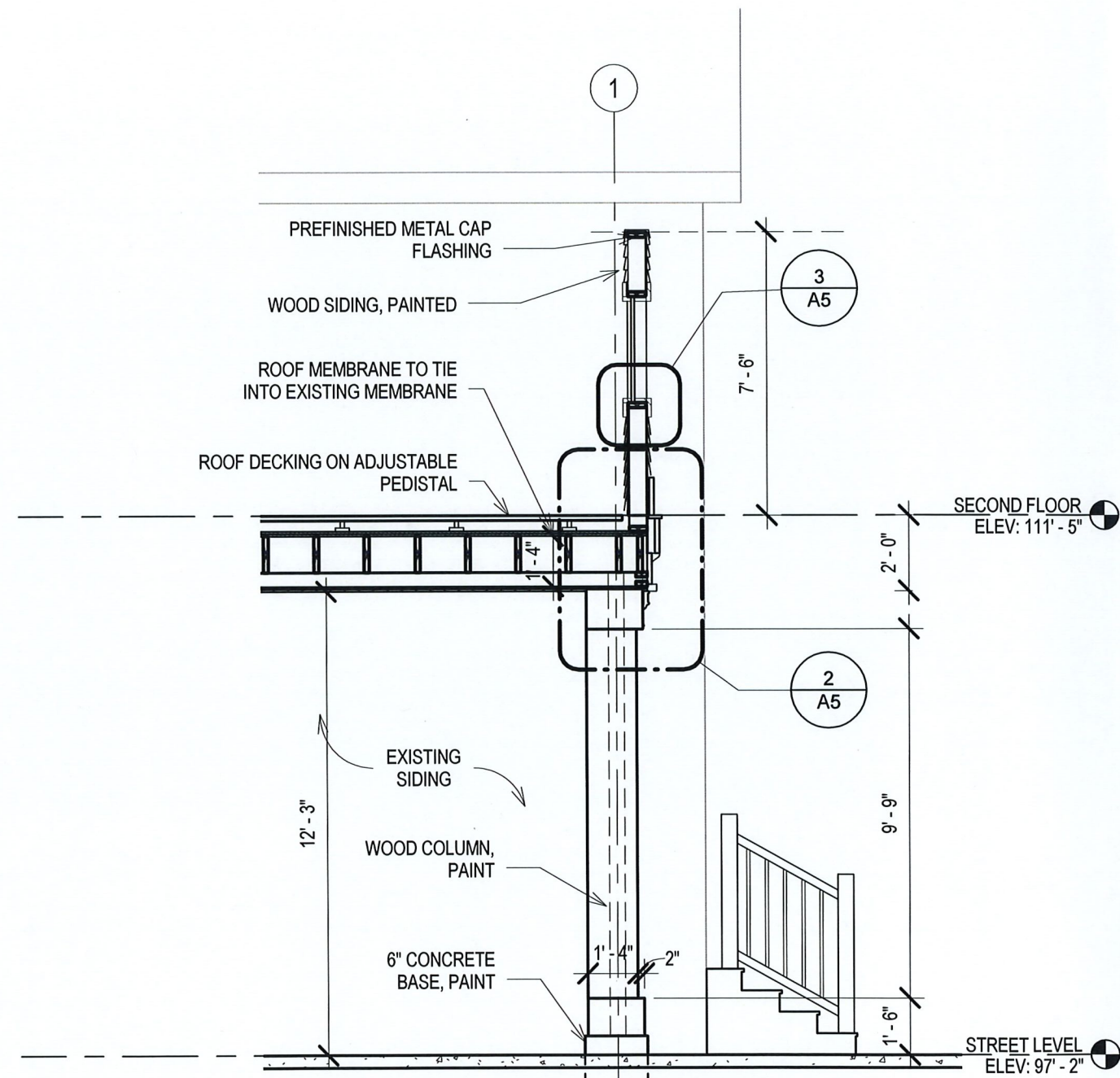
1 SECTION THROUGH ADDITION Scale: 1/4" = 1'-0"
