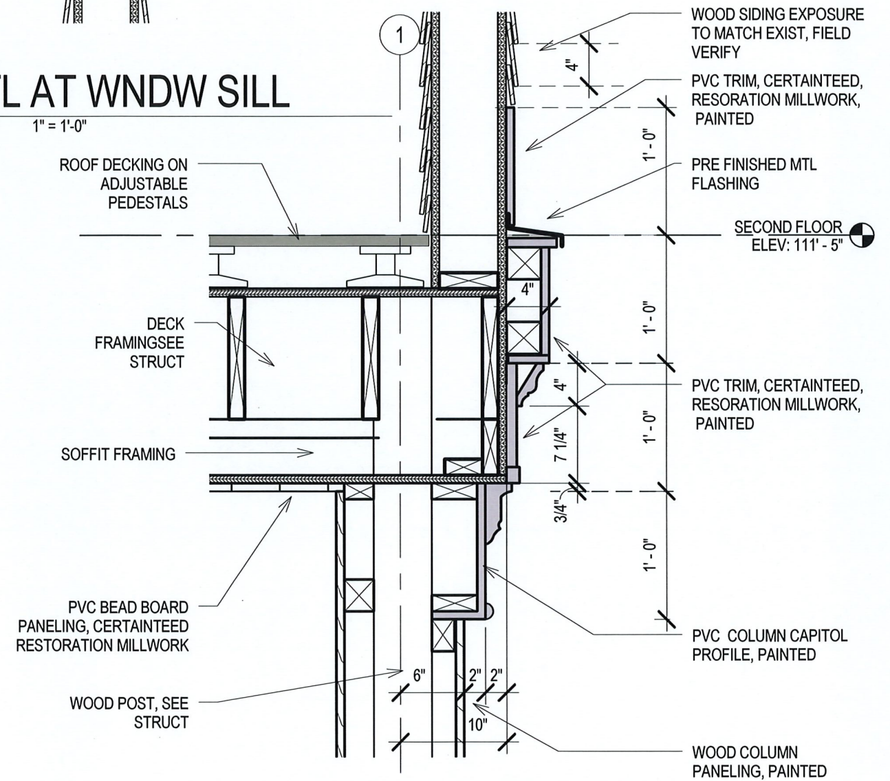
2 DETAIL AT FASCIA Scale: 1" = 1'-0"
