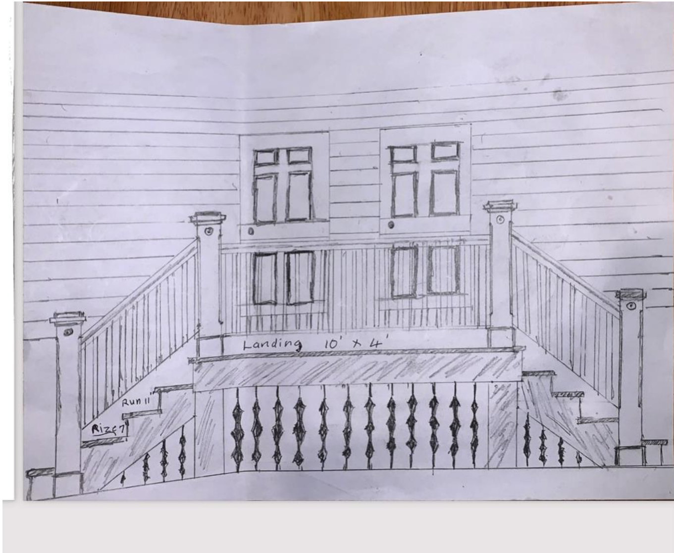
Proposed Lloyd Street elevation.
