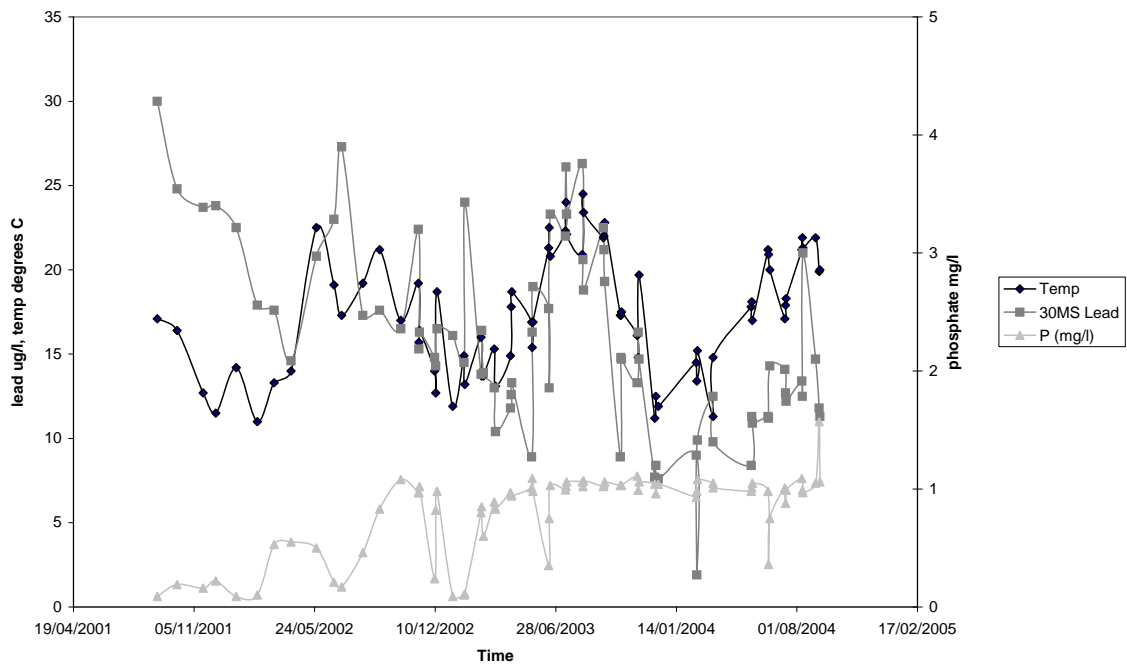
Figure B.10.6 Lead and phosphate date for customer property no. 5 for 2001-2004
