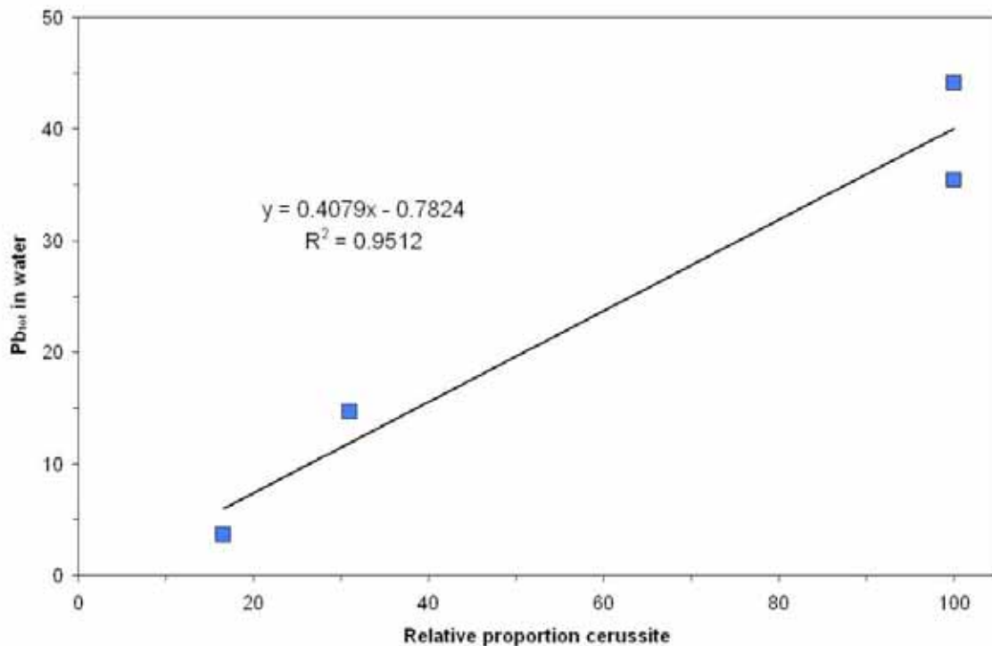
Figure F.18 Relationship of Average Total Lead Measured in Sequential Samples to the Relative Proportion of Cerussite Among the Scale Minerals (the dominant mineral is assigned a value of 100 percent and the other minerals scaled accordingly by peak intensity)
