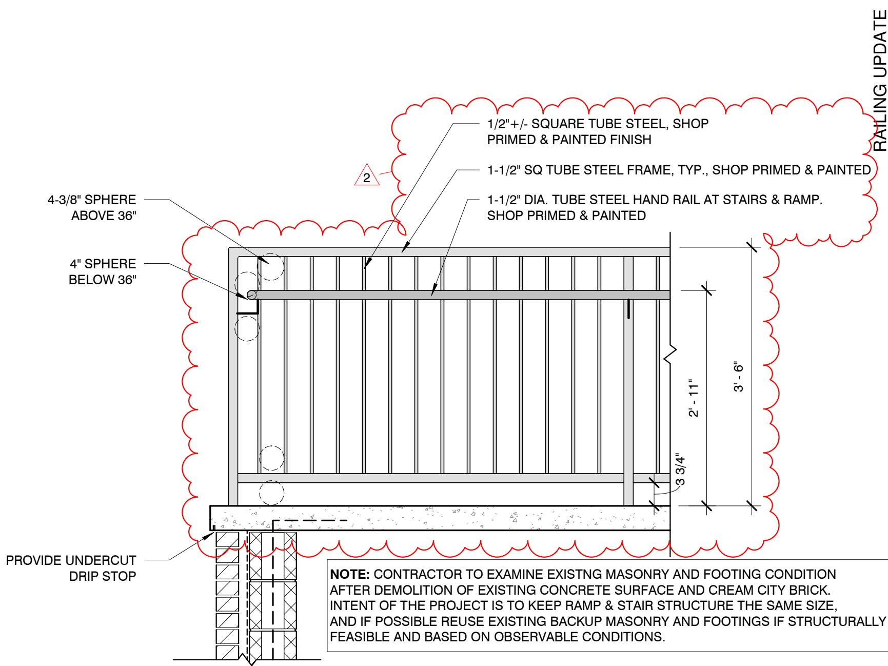
1 TYPICAL RAILING DETAIL CB1-A1 3/4" = 1'-0"
