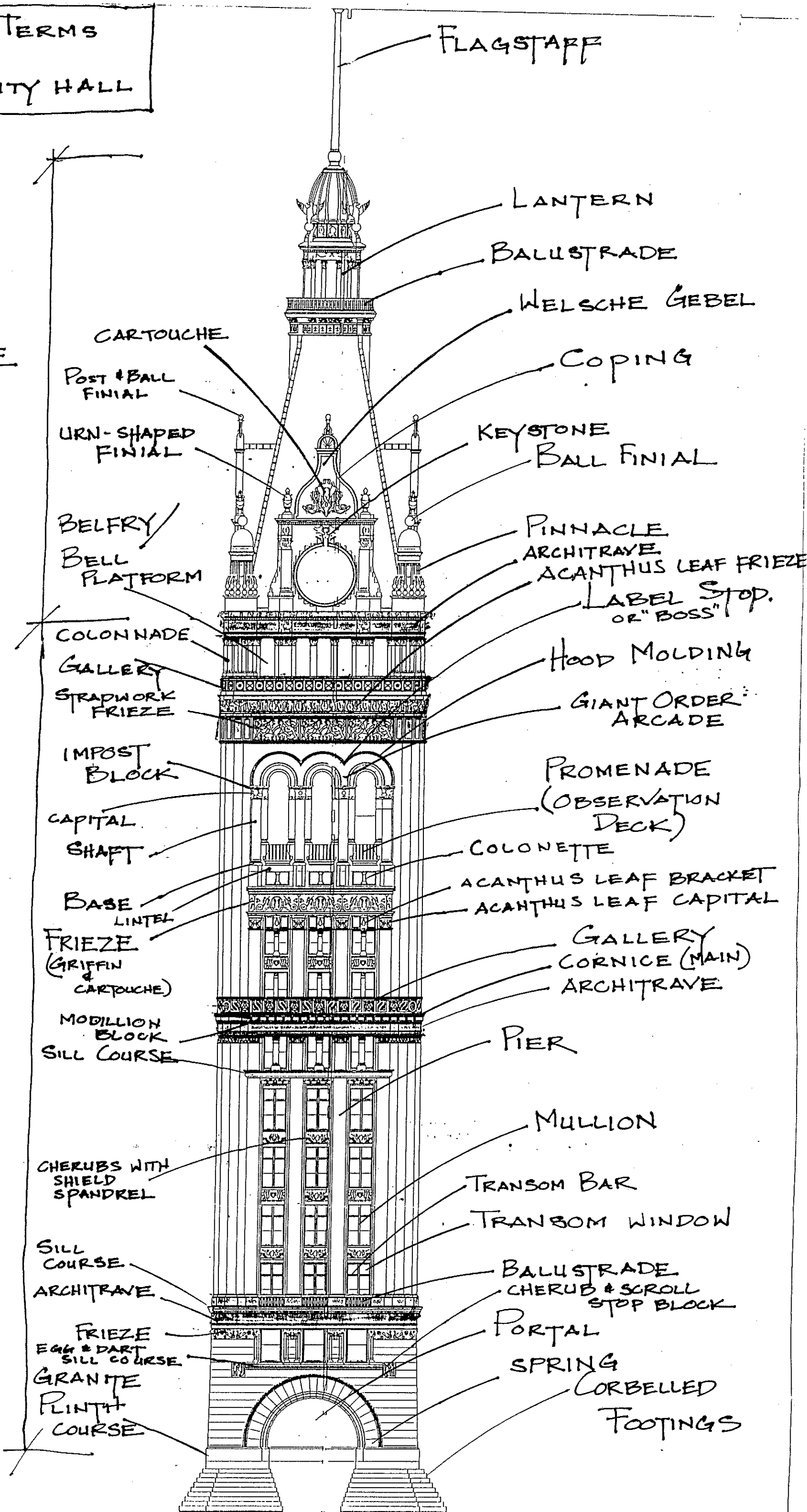
SOUTH TOWER SOUTH ELEVATION
