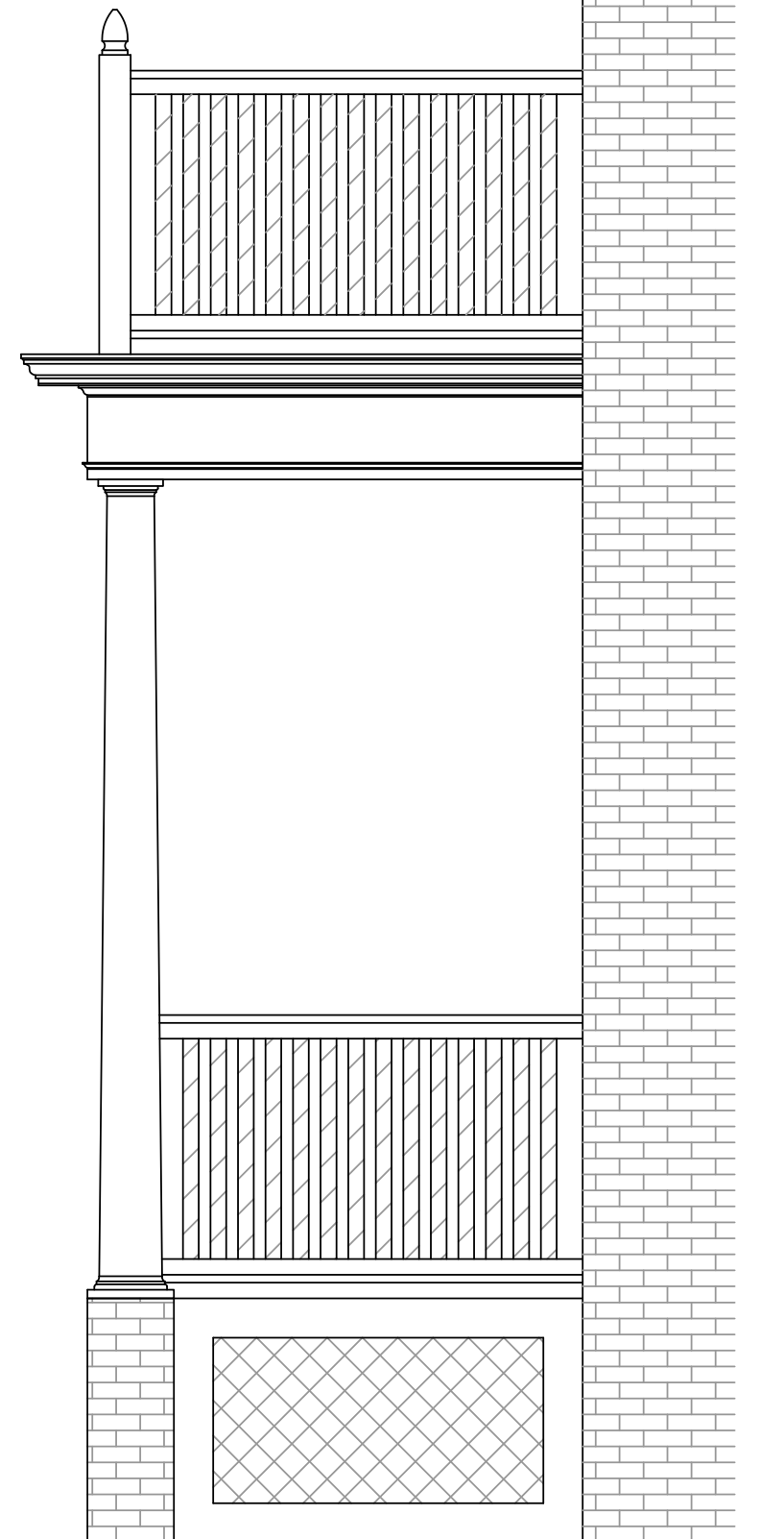
Side Elevation
