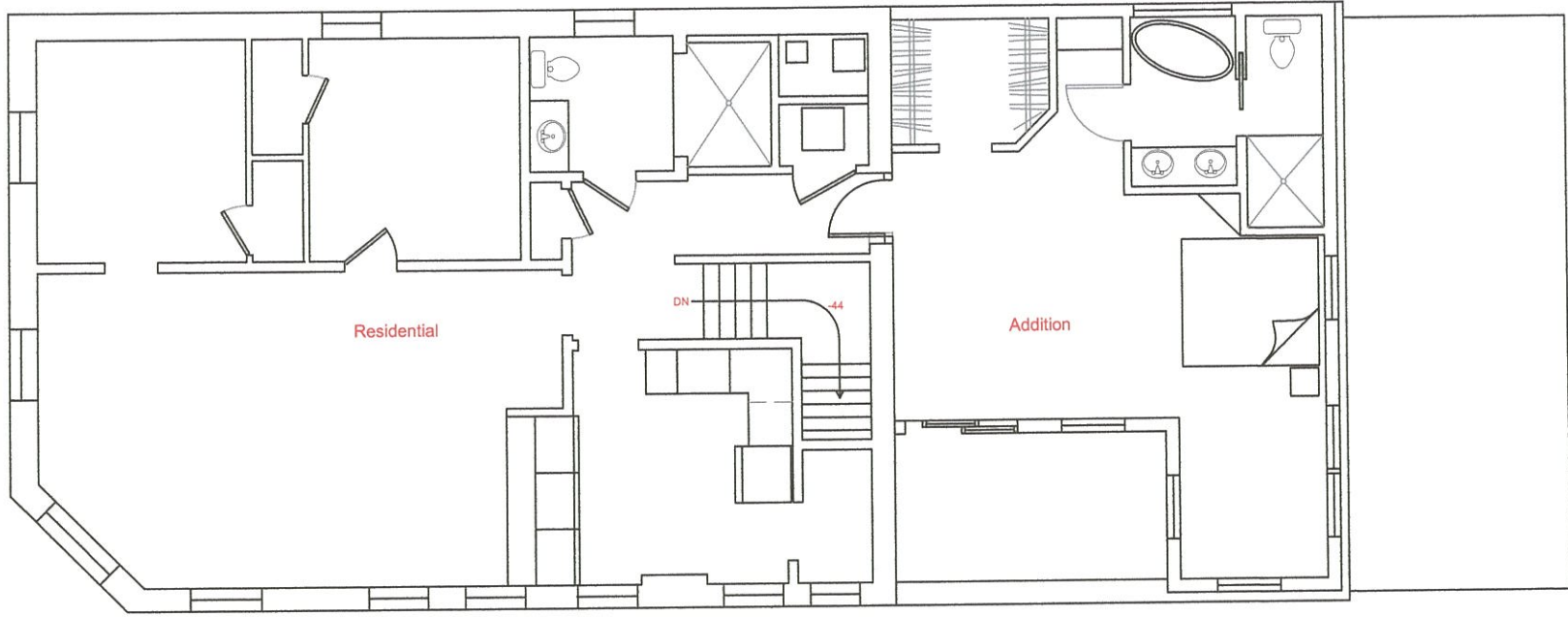
Second Floor
