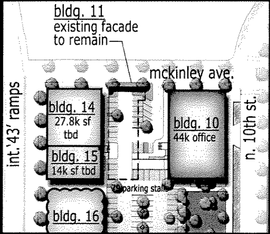
SITE PLAN
