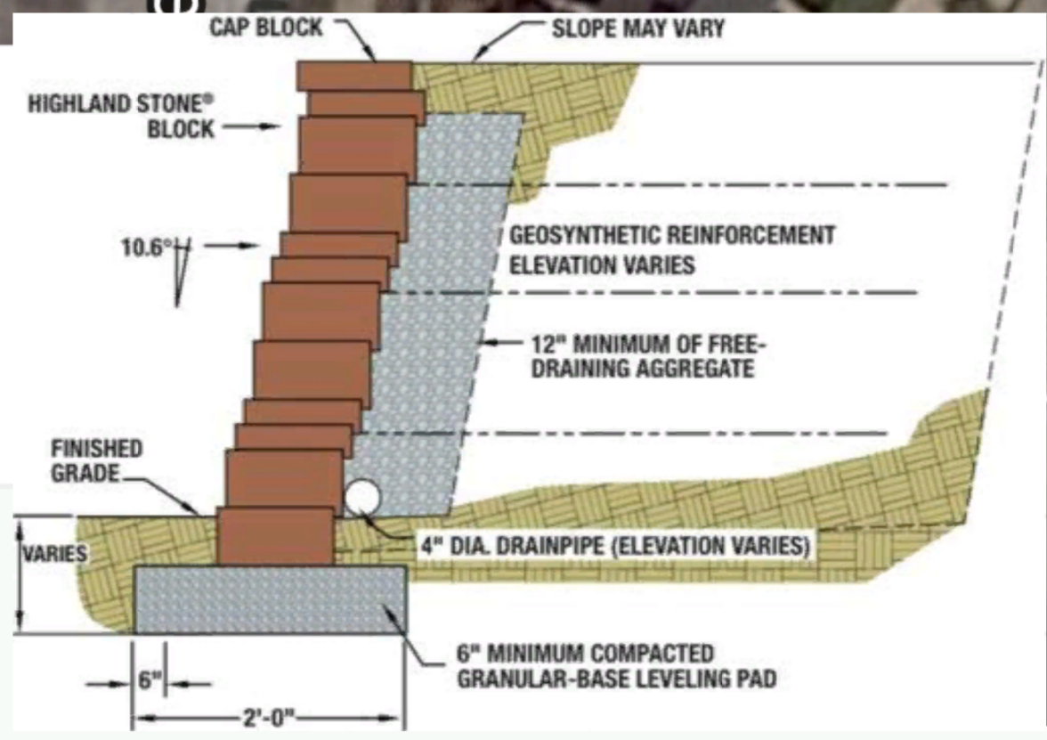
Geo-Grid Example
