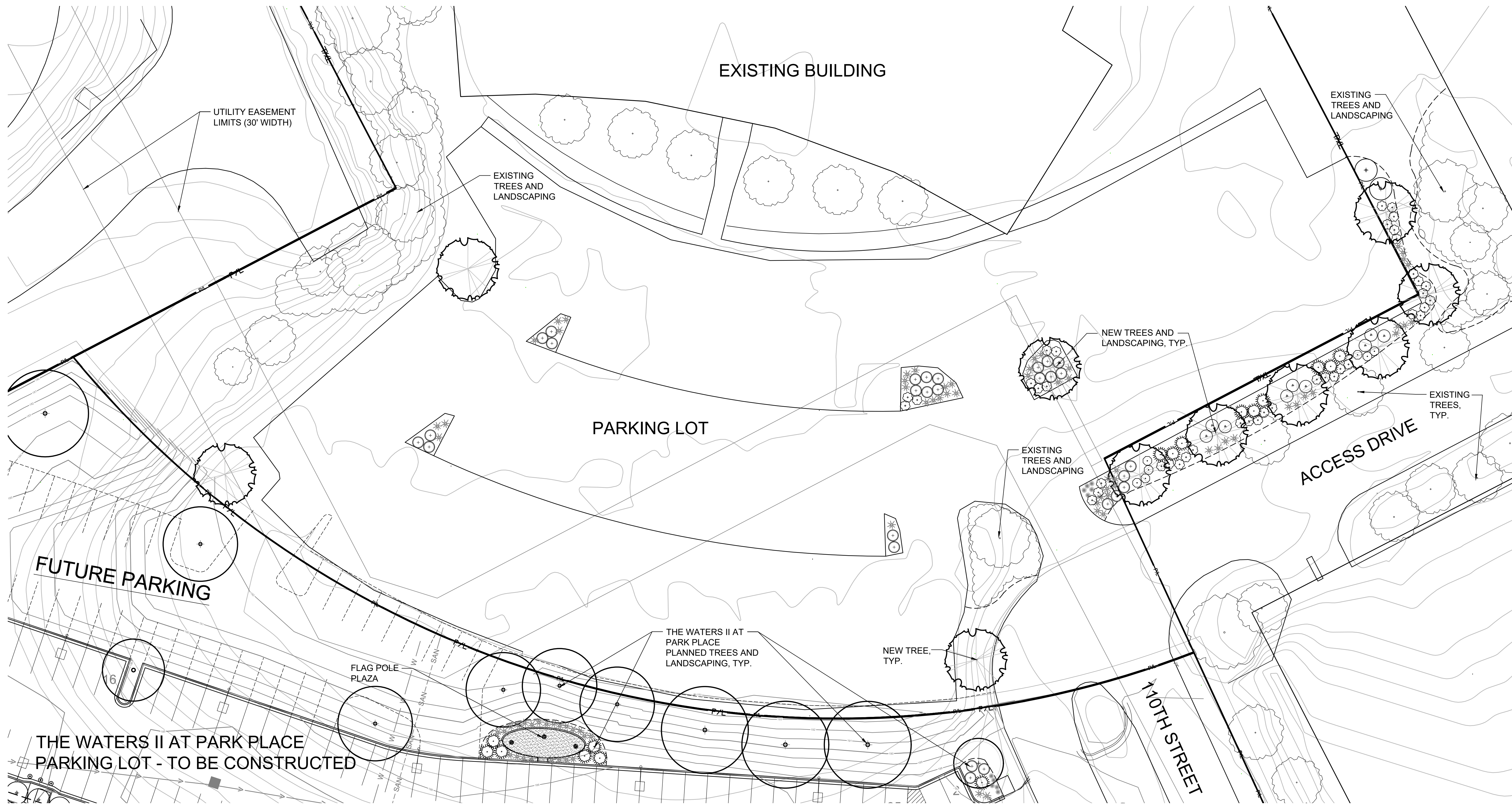
1 LANDSCAPE CONCEPT PLAN L100 SCALE: 1" = 20'
