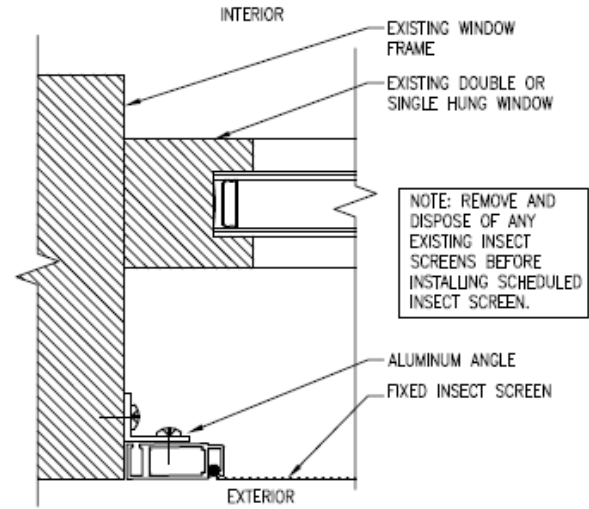
INSECT SCREEN - JAMB DETAIL (DOUBLE & SINGLE-HUNG)
