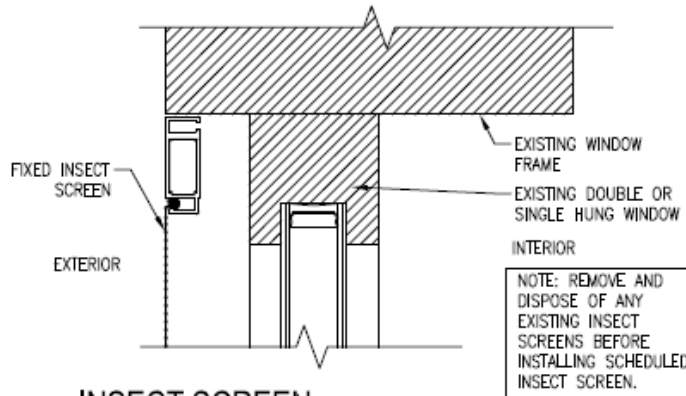
INSECT SCREEN - HEAD DETAIL (DOUBLE & SINGLE-HUNG)
