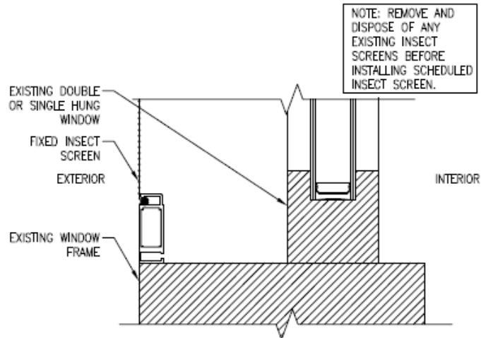
INSECT SCREEN - SILL DETAIL (DOUBLE & SINGLE-HUNG)
