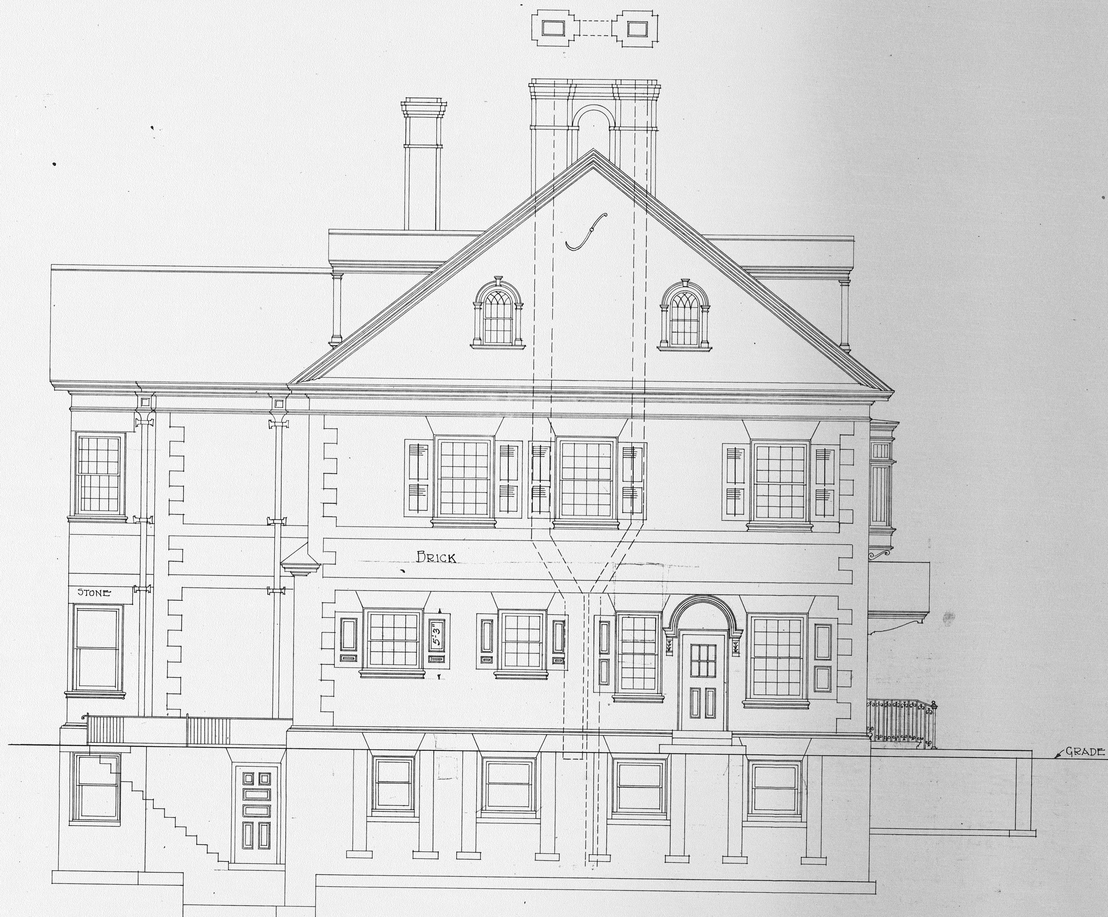
NORTH ELEVATION SCALE - 1/4" = 1'-0"
