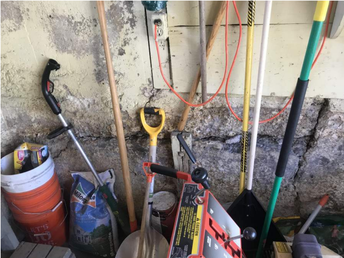
Photo 10 - West Elevation of the Interior of the Existing Garage Showing Deterioration of the Structure
