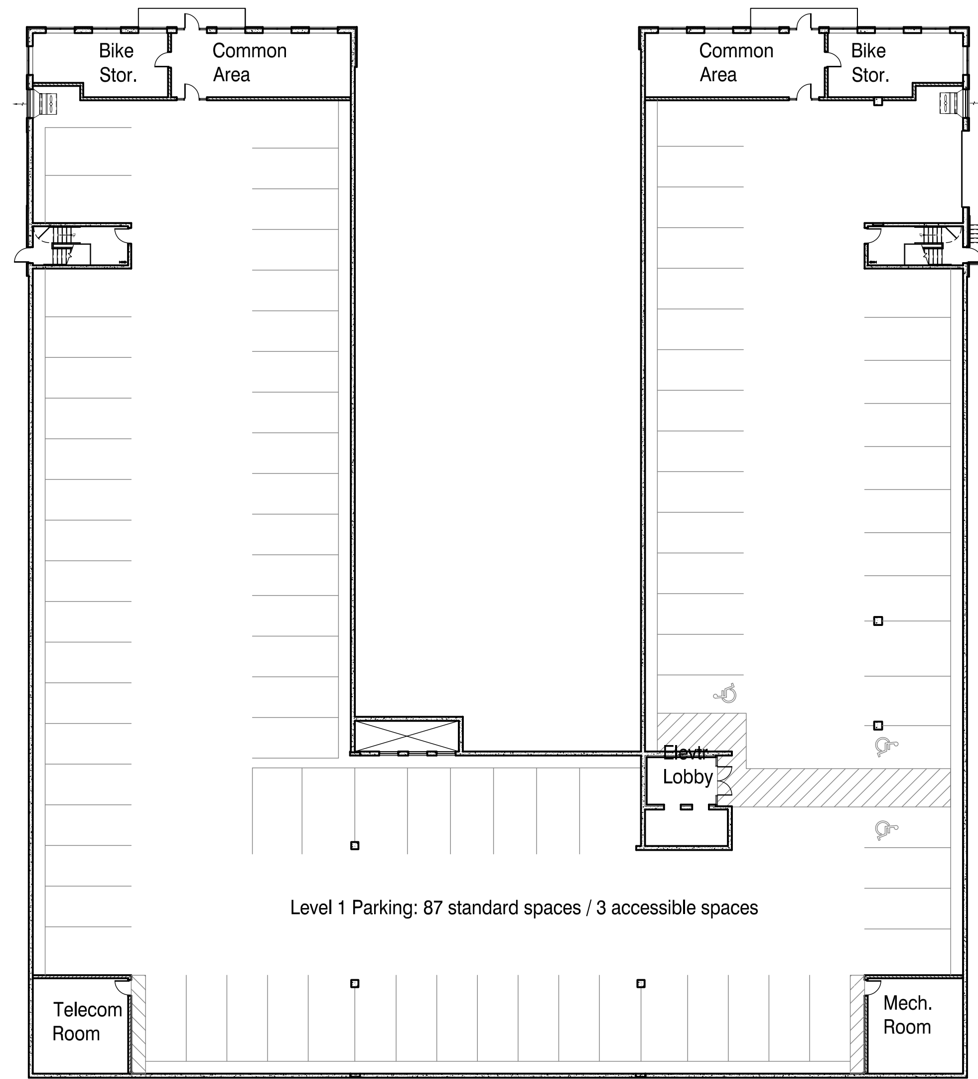
1 LL BASEMENT BUILDINGS 1 AND 2 SCALE: 1"=20'-0"
