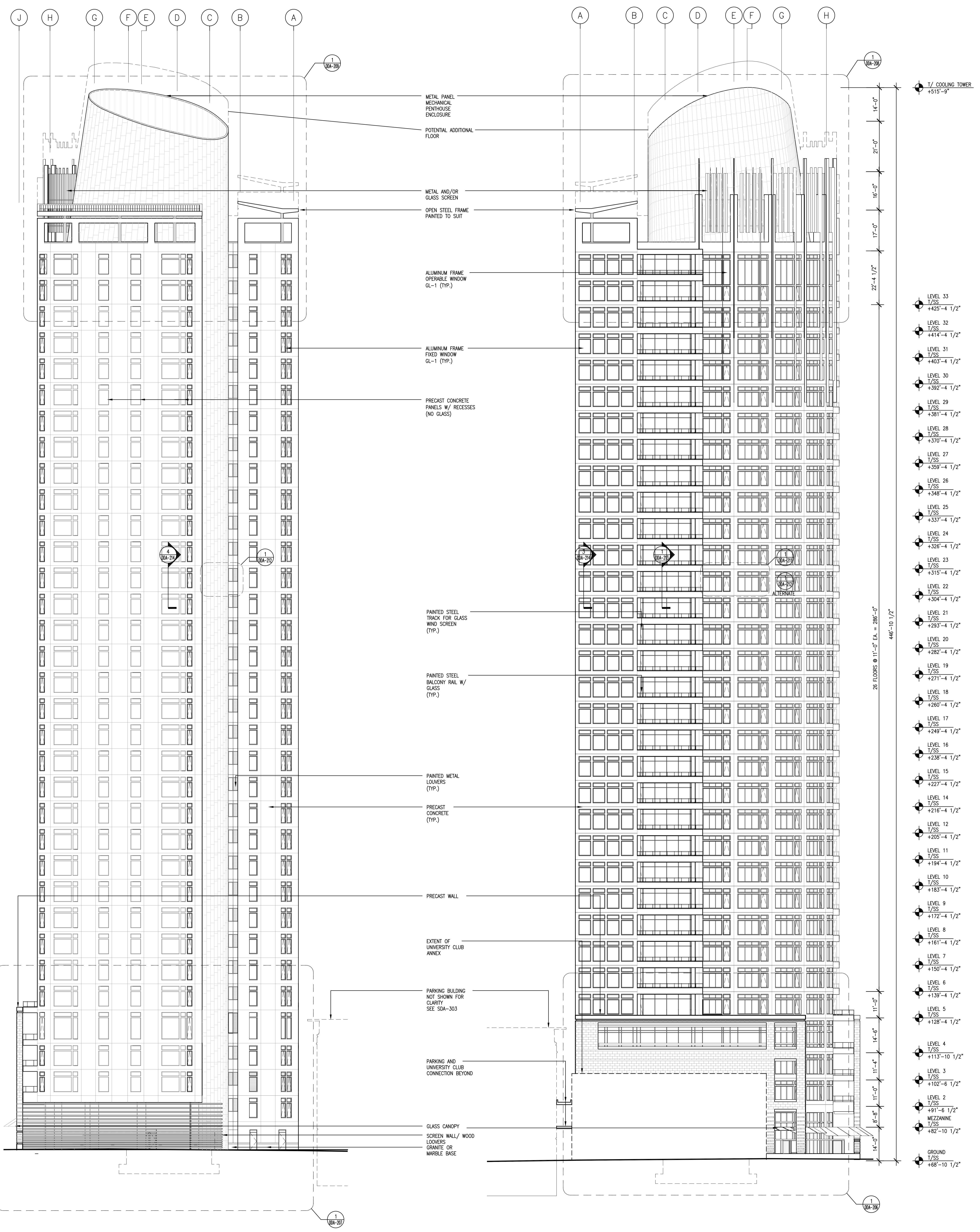
2 NORTH BUILDING ELEVATION SCALE: 1/16" = 1'-0"
