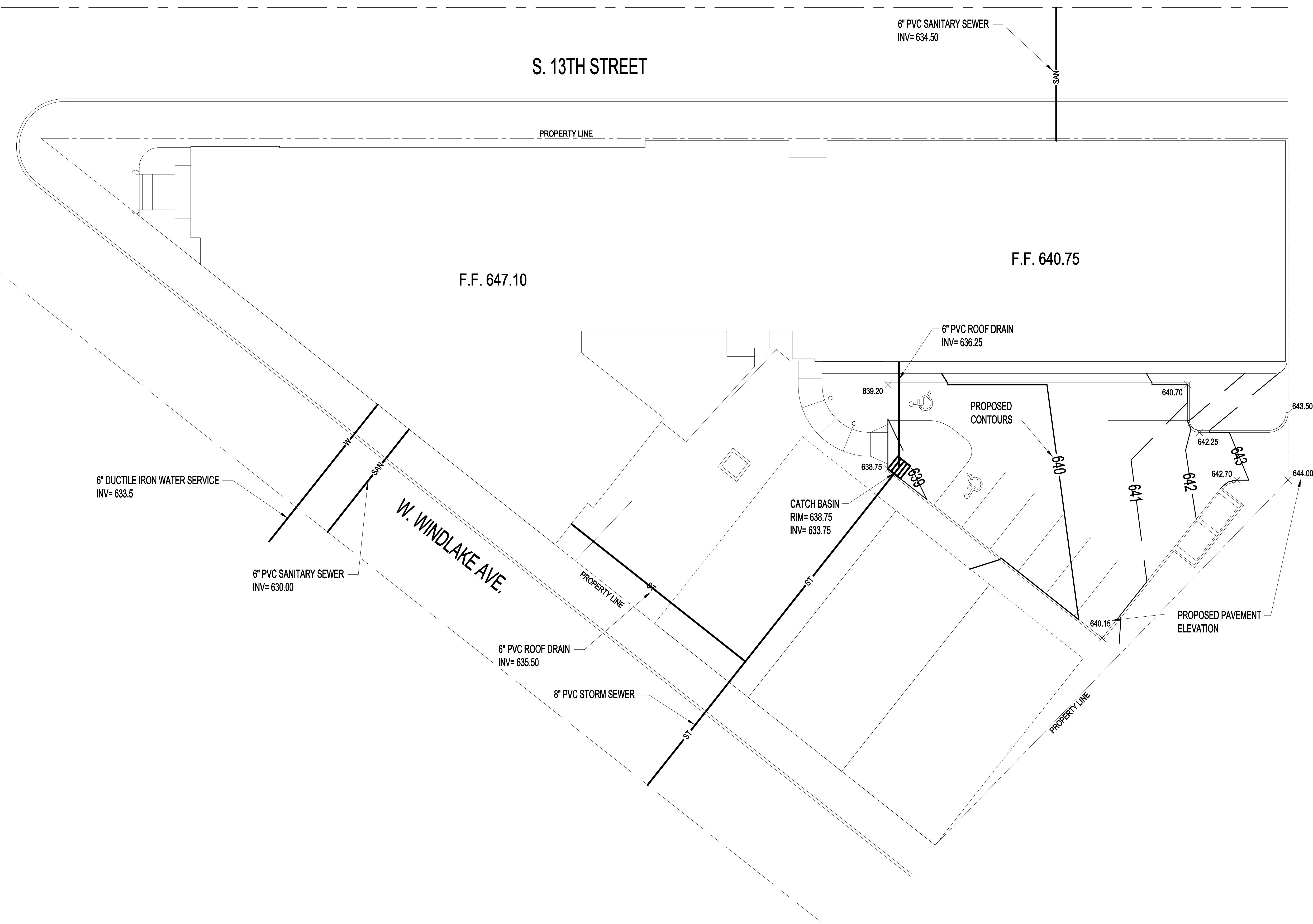
1 SITE GRADING & UTILITY PLAN
