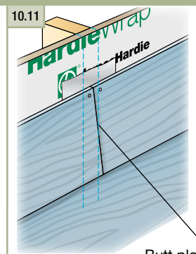
Butt planks with moderate edge contact
