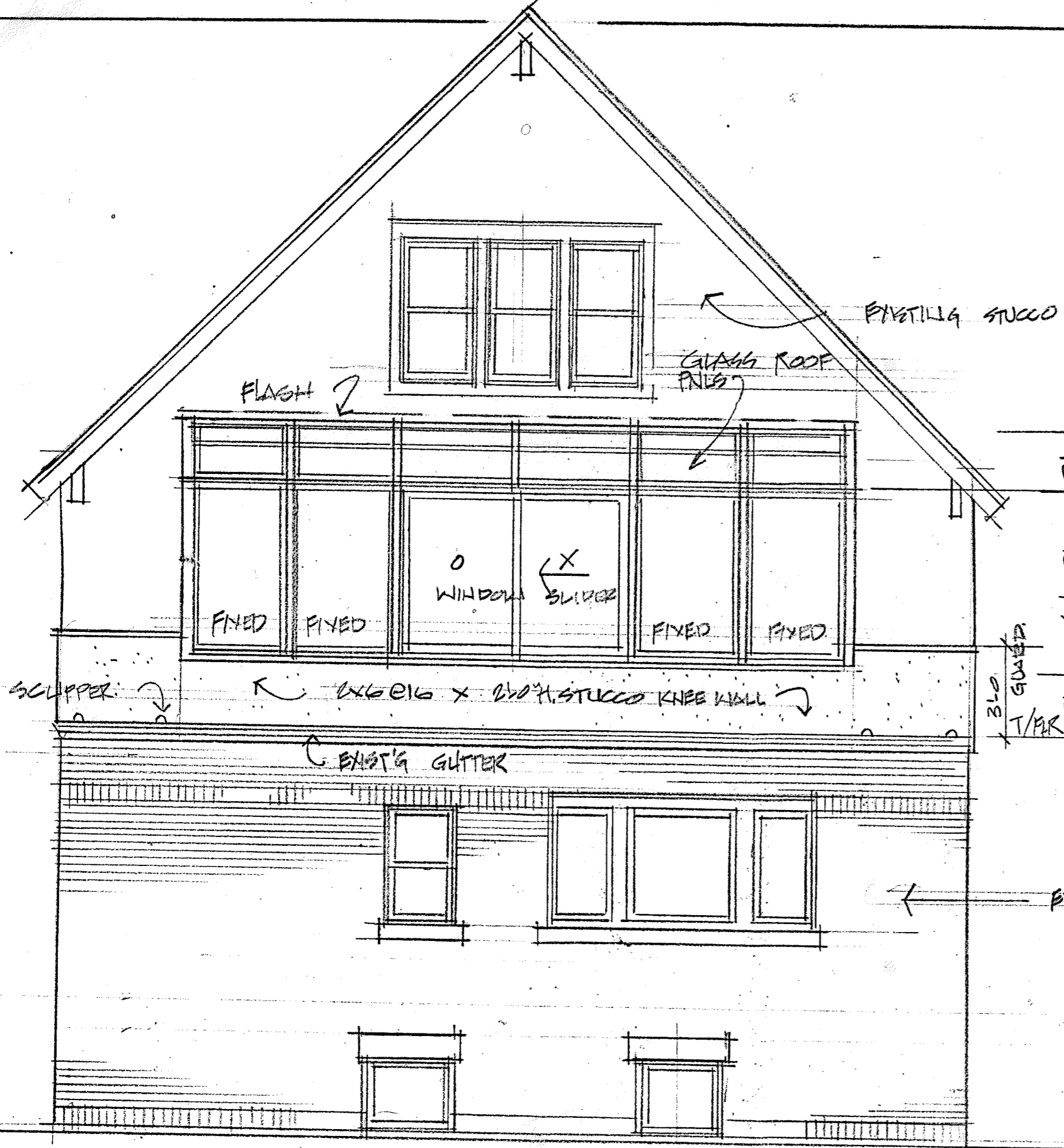
REAR (B-WALL) ELEVATION
