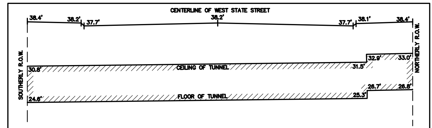
PROFILE OF SUBSURFACE TUNNEL LOOKING WEST
