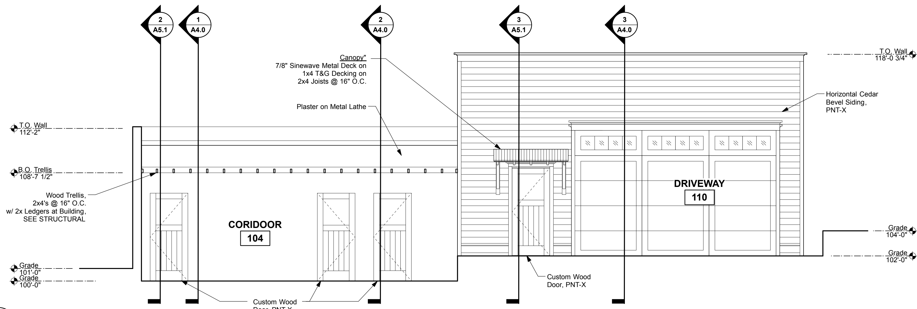
2 Building Elevation - Interior West
